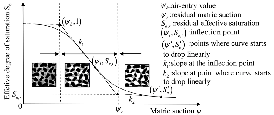
Figure 3. Typical soil-water characteristic curve [12].
