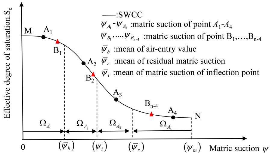
Figure 2. Illustration of control measuring points and additional measuring points.
