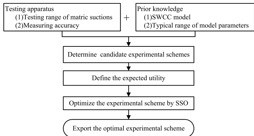
Figure 1. One-stage Bayesian experiment design optimization (OBEDO) framework for measuring SWCC.
