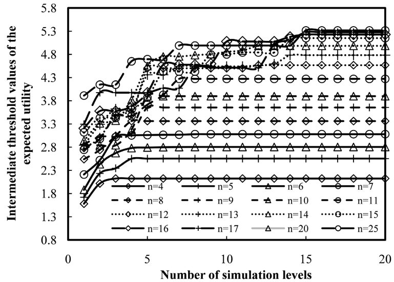
Figure 5. Evolution of SSO for different numbers of measuring points.
