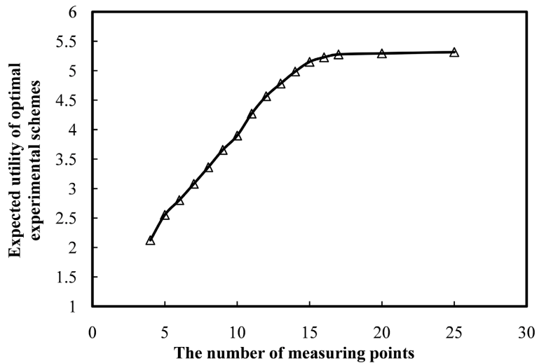
Figure 6. Expected utility with different number of measuring points.
