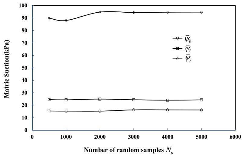
Figure 4. Determination of \bar{\psi}_b , \bar{\psi}_i and \bar{\psi}_r based on prior knowledge in the illustrative example.
