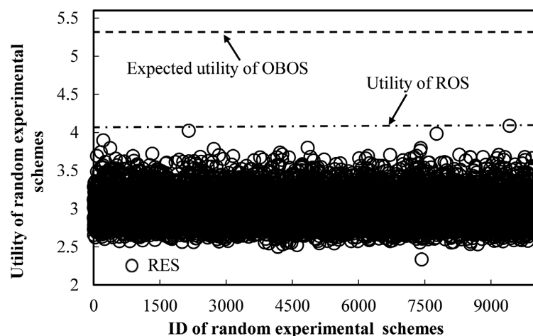
Figure 8. Utility of random experimental schemes.
