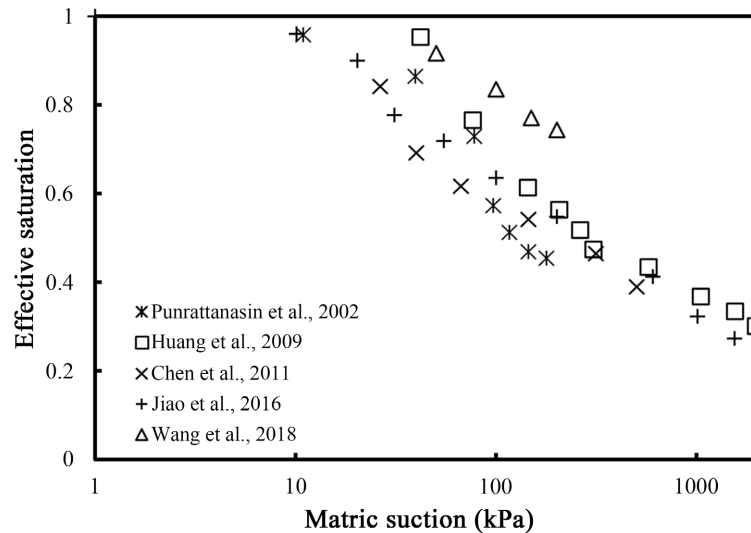
Figure 7. SWCC measured data of loess.
