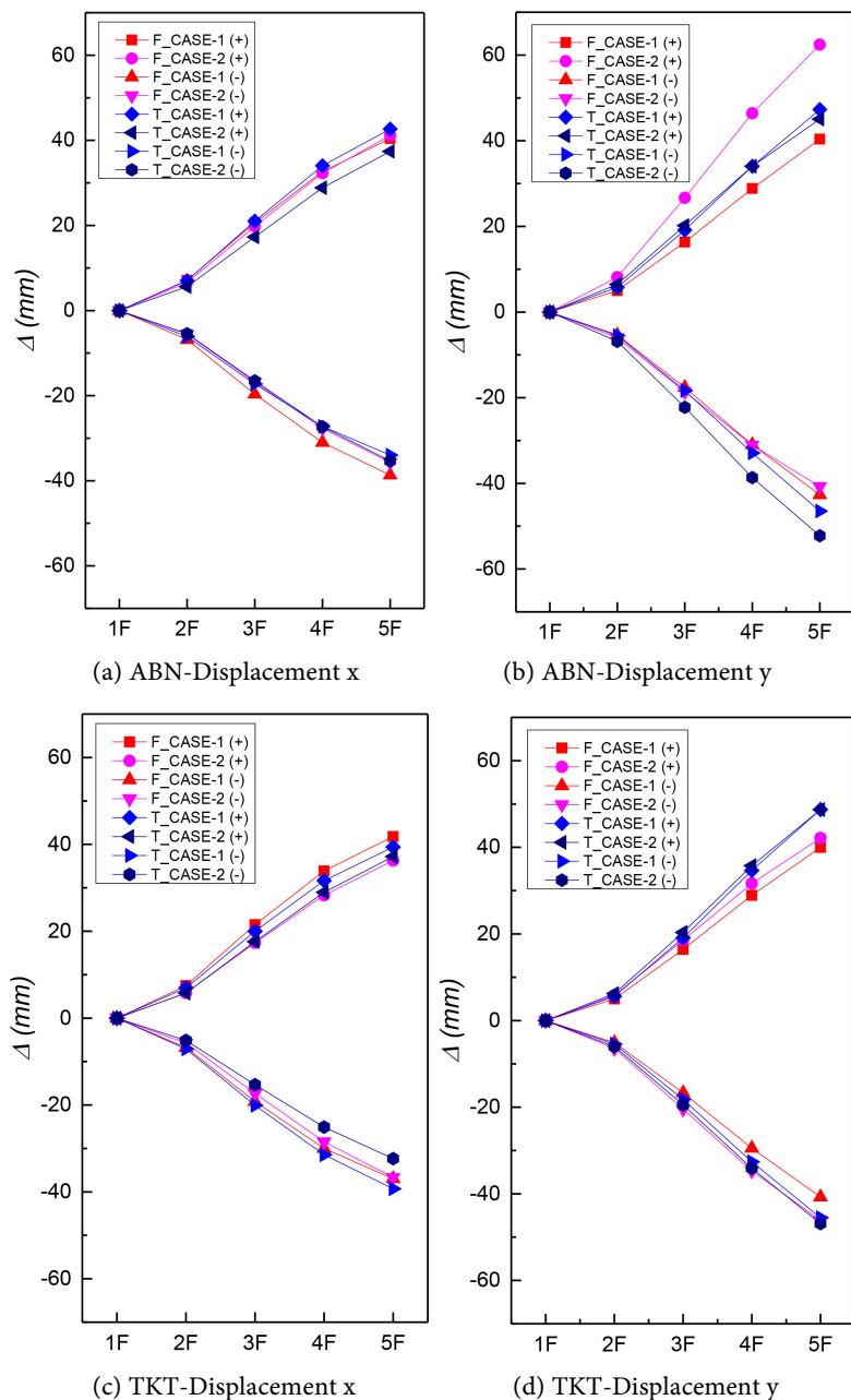
Figure 11. Average displacement.
