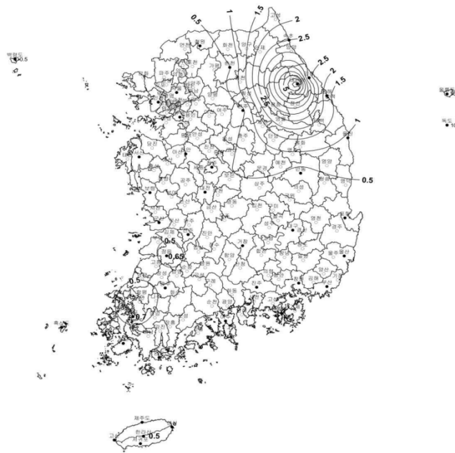
Figure 4. Design of the snow load (KBC 2016).
