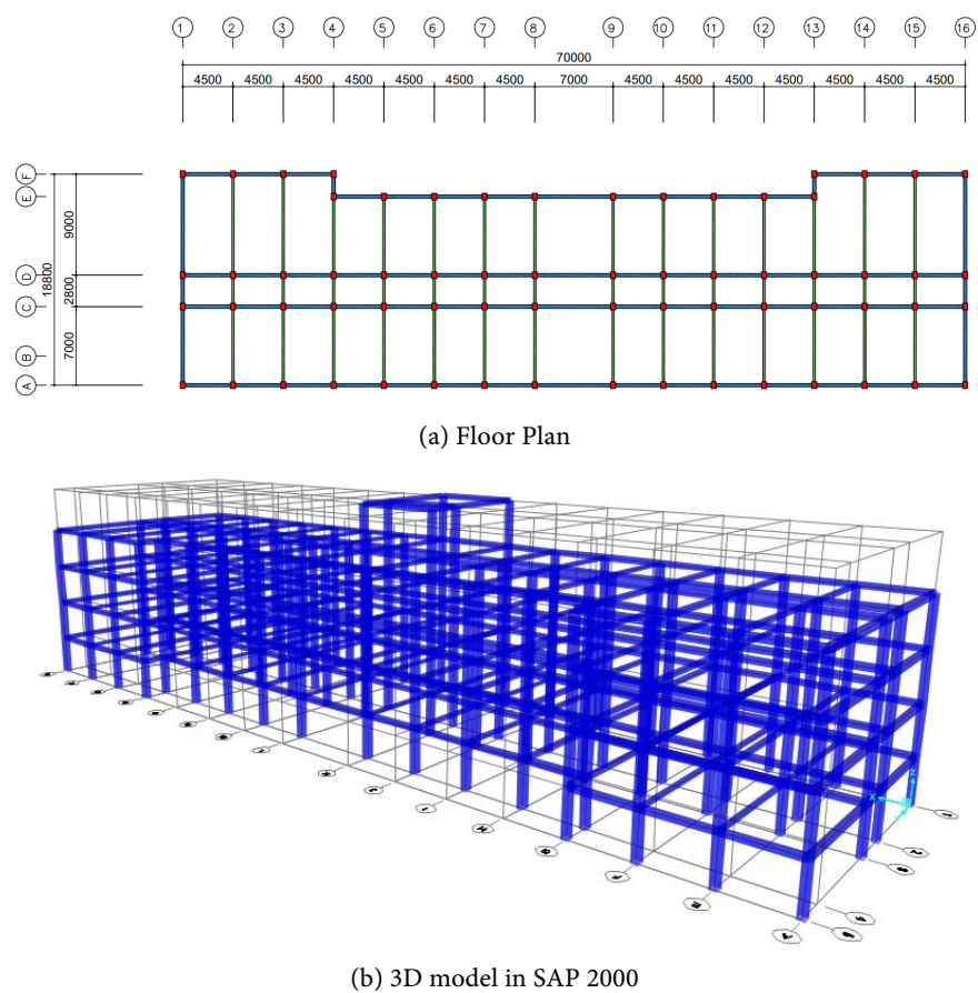
Figure 2. Design of the specific RC frame structure.
