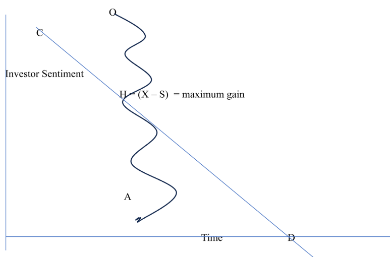
Figure 7. Optimal price for a cryptocurrency put buyer.
