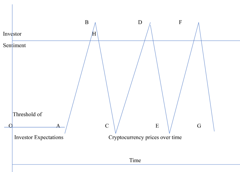
Figure 5. The Optimization Function for Cryptocurrency Futures Prices.
