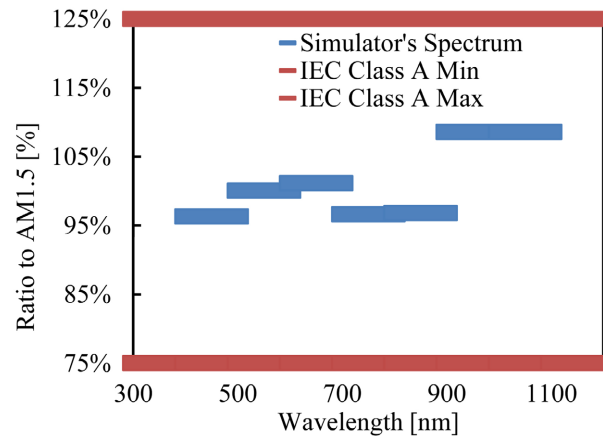
Figure 5. Evaluation of the simulator's spectrum versus AM1.5 at 200 \text{ Wm}^{-2} .
