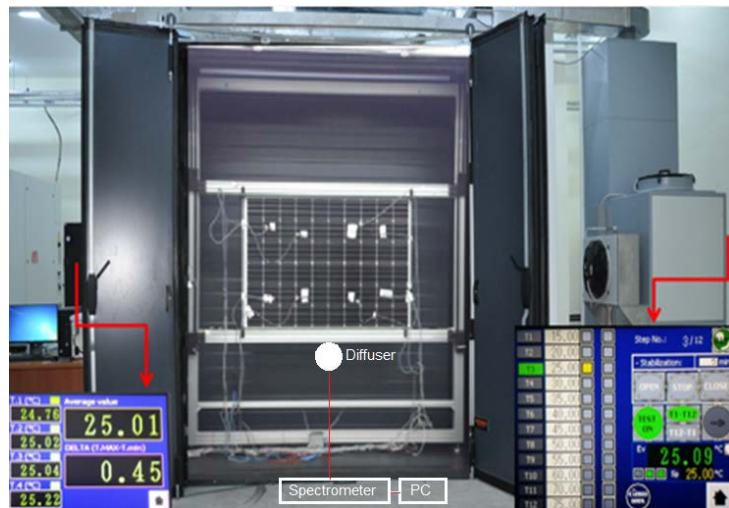
Figure 1. Thermal chamber integrated solar simulator system.
