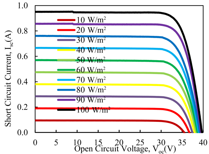
Figure 11. I_{sc} - V_{oc} curves of a monocrystalline PV module.
