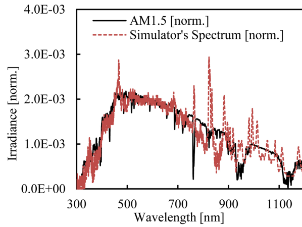
Figure 2. Spectral distribution of simulator versus AM1.5 at 1000 \text{ Wm}^{-2} .
