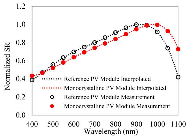
Figure 14. Spectral responsivity of monocrystalline PV module.
