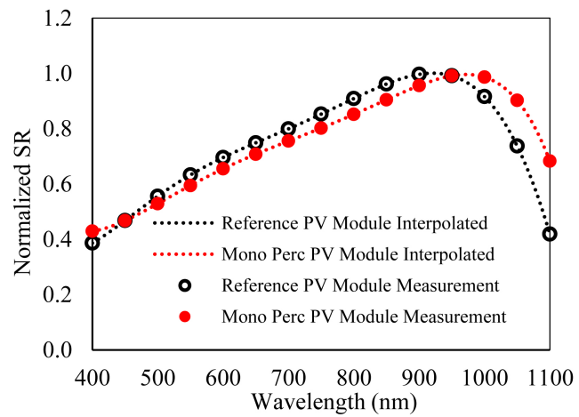
Figure 16. Spectral responsivity of MonoPerc PV module.
