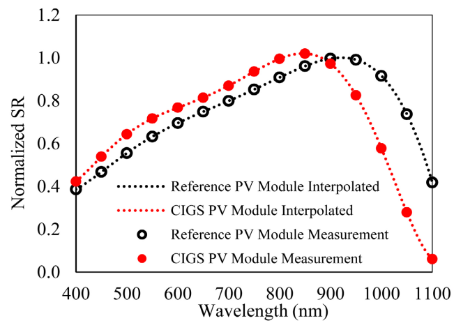
Figure 17. Spectral responsivity of CIGS_1 PV module.
