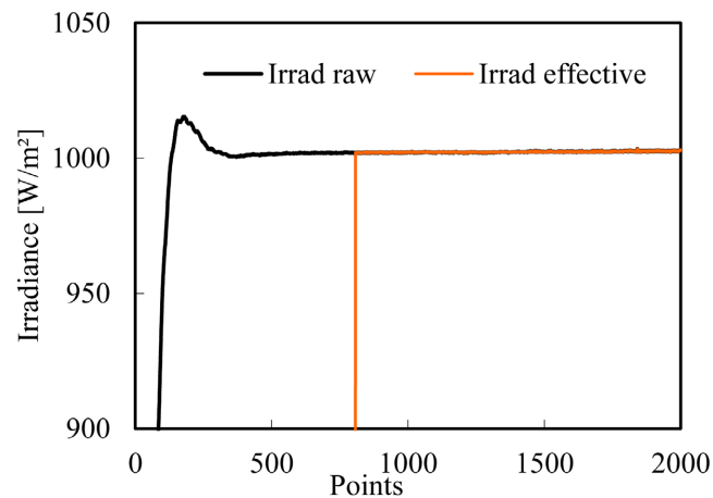
Figure 9. Temporal instabilities of solar simulator regulated by control cell.
