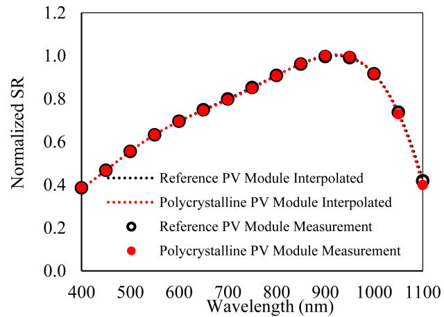
Figure 13. Spectral responsivity of polycrystalline PV module.
