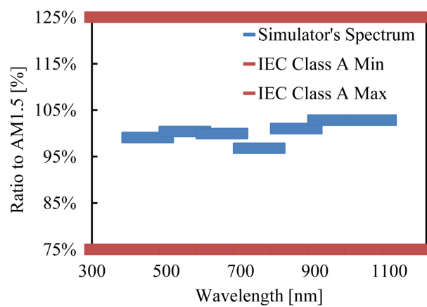
Figure 4. Evaluation of the simulator's spectrum versus AM1.5 at 1000 \text{ Wm}^{-2} .
