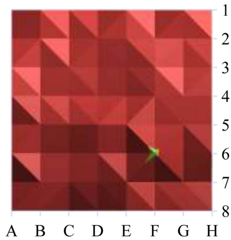
Figure 6. Non uniformity measurement of solar simulator as a function of irradiance at 1000 \text{ Wm}^{-2} .
