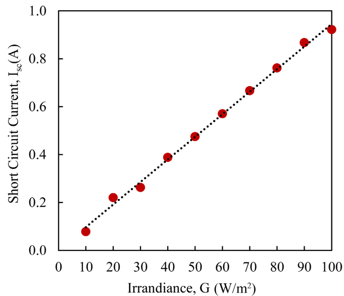
Figure 12. I_{sc} - G curves of a monocrystalline PV module.
