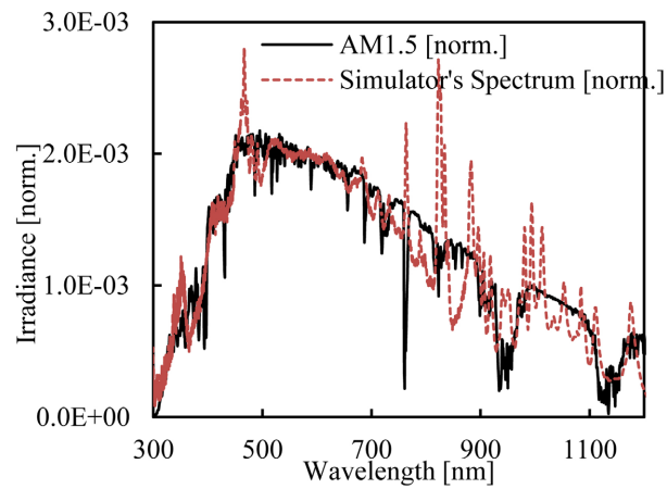
Figure 3. Spectral distribution of simulator versus AM1.5 at 200 \text{ Wm}^{-2} .
