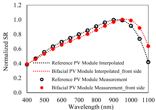
Figure 15. Spectral responsivity of bifacial PV module.
