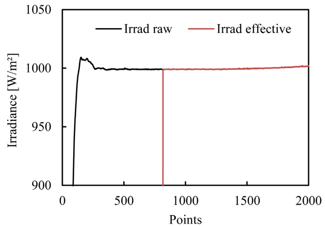
Figure 8. Temporal instabilities of solar simulator regulated by optical sensor.
