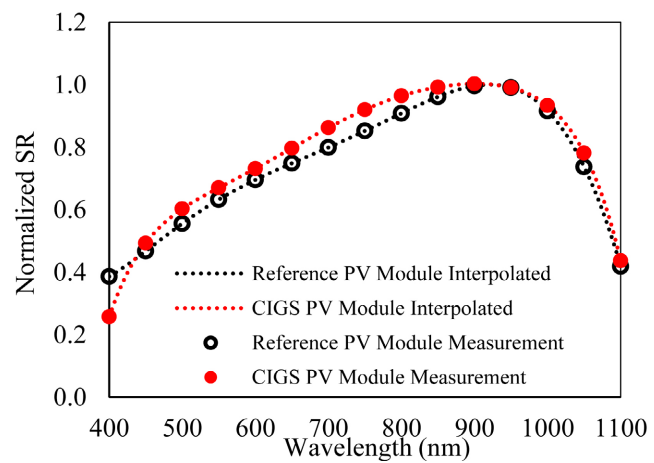
Figure 18. Spectral responsivity of CIGS_2 PV module.
