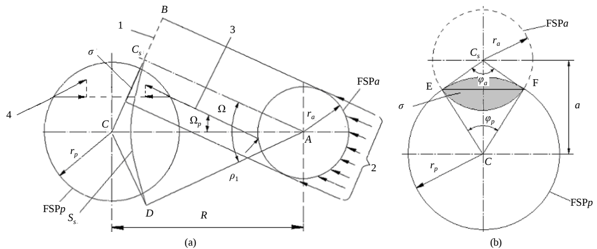
Figure 1. (a) Scheme for the calculation of the shadow force of gravity acting on the FSP. The passive FSPp is shadowed, from the right side, by the active FSPa from the flows of fations 2 directed within the limits of the solid angle element d\Omega of the solid angle \Omega (unidirectional flows having energy density \varepsilon_G^* ). Only flows 3, reflected from FSPa, fall on the FSPp under a plane angle \Omega_p , from the right side. Analogous flows, 4, act on FSPp from the left side; (b) Cross-section along BCD (on (a)). The force element is proportional, in modulo, to the area of the shadow element, \sigma , that falls on the cross-section BC of the passive FSPp from the active FSPa (a). C_s is the shadow center; r_a and r_p are radii of active and passive FSPs.
