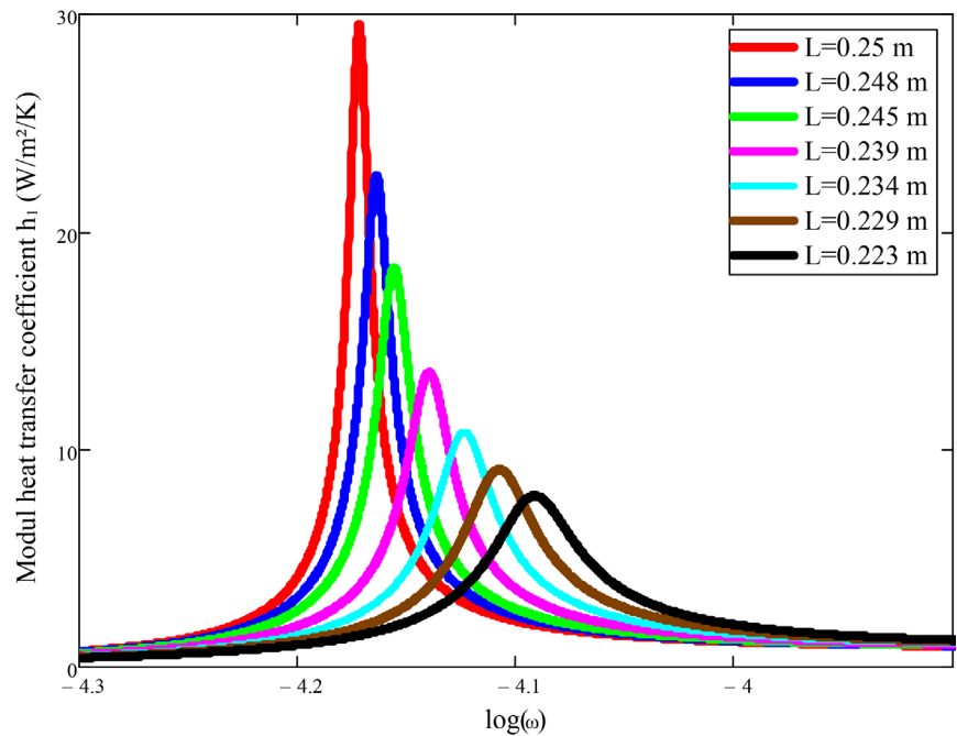
Figure 3. Evolution of h_1 as function excitation pulse \omega (rad.s -1 ); influence of thickness.
