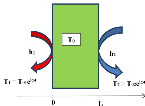
Figure 1. Wall typha.
