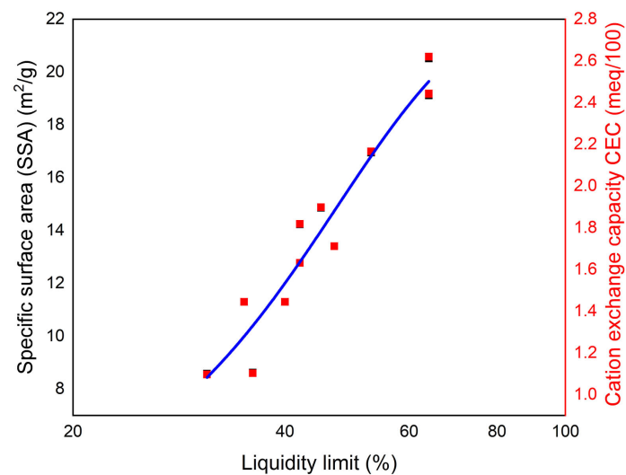
Figure 13. Evolution of the specific surface area and the cation exchange capacity in function of the liquidity limit.
