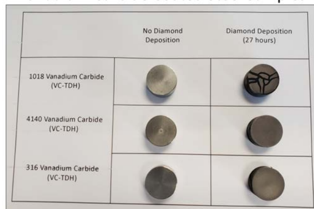
Figure A3. Layout of diamond-coated steel samples with VC interlayer.
