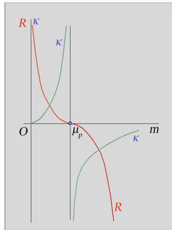
Figure 1. Particle radius and curvature.
