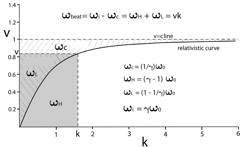
Figure 2. Elementary particle's internal frequencies when on relativistic curve.
