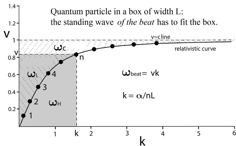
Figure 3. Elementary particle's quantized frequencies when on relativistic curve.
