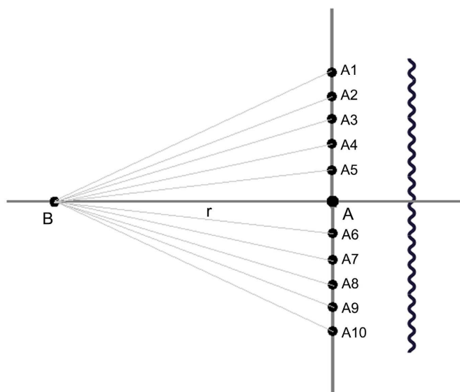
Figure 1. Many cases in 4-dimensional space map to the same situation in 3-dimensional space.
