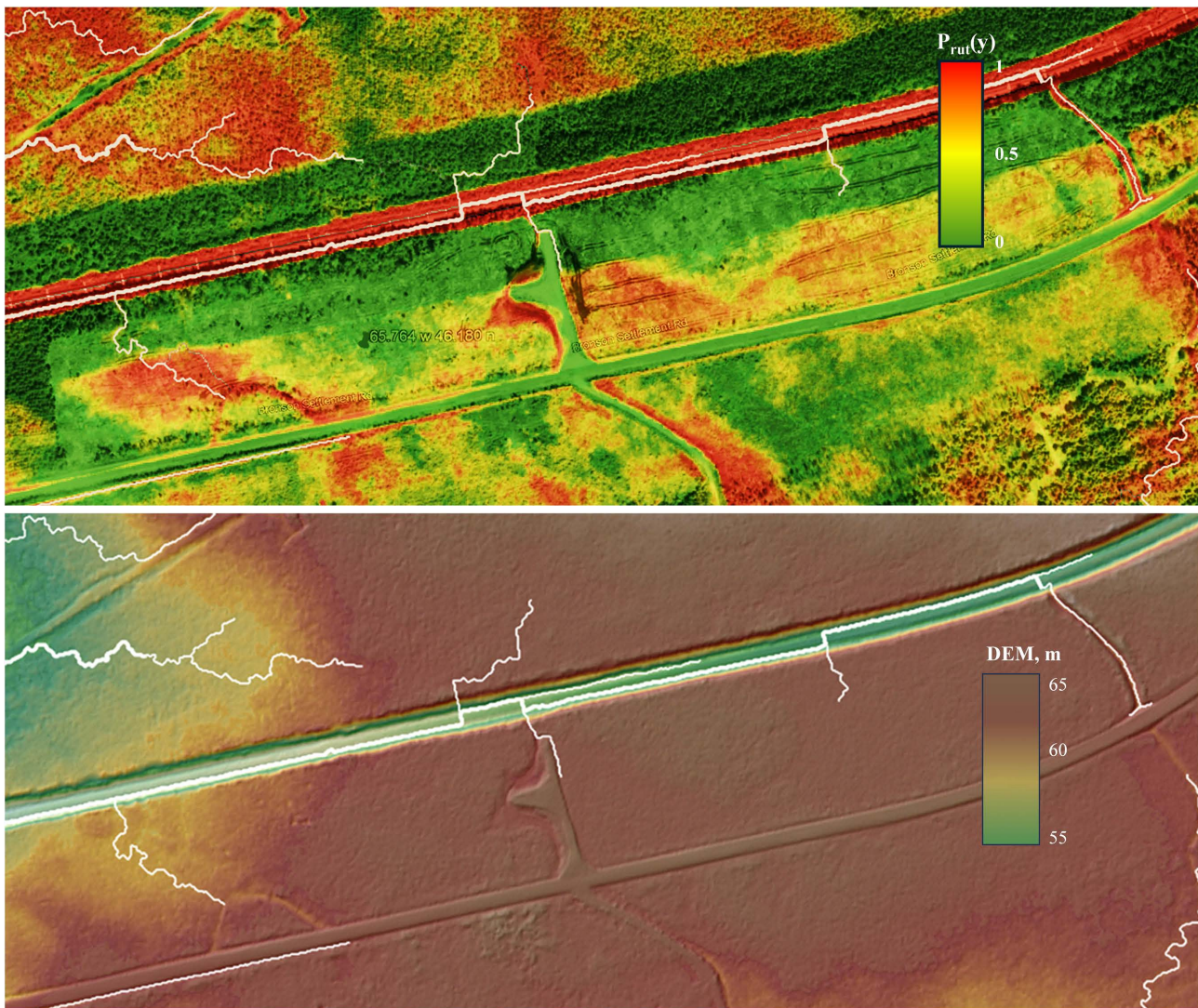
Figure 10. Top: Example of a false P_{\text{rut}}(y) no-rut projection situation as found on a flat terrain within 30 m due to the impact of the 5-m incised train track on the TPI calculations. In contrast, also note the general low to absent influence of the slightly elevated road running parallel south of the train track. Location: 46.180, -65.764; Google Earth Image: June 2019; Bottom: LiDAR-DEM 2015.
