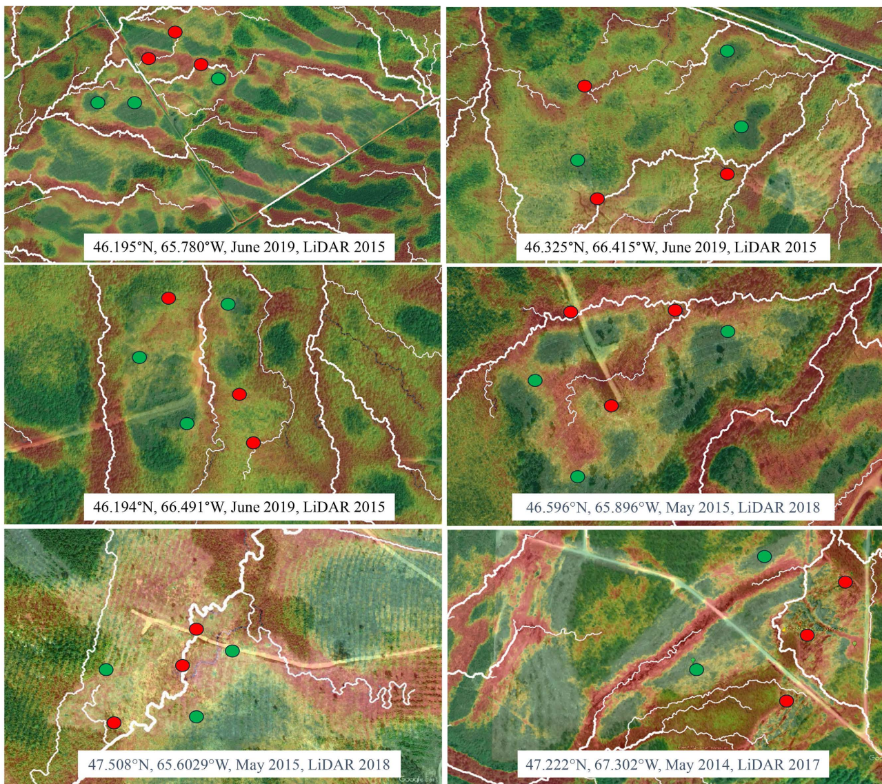
Figure 6. Overlay of the 0 (green) to 1 (red) rut occurrence probability pattern underneath the marked rut (red) and no-rut (green) locations on the image panels in Figure 2 , with yellow-colored P_{rut}(y) \approx 0.5 transition zones.
