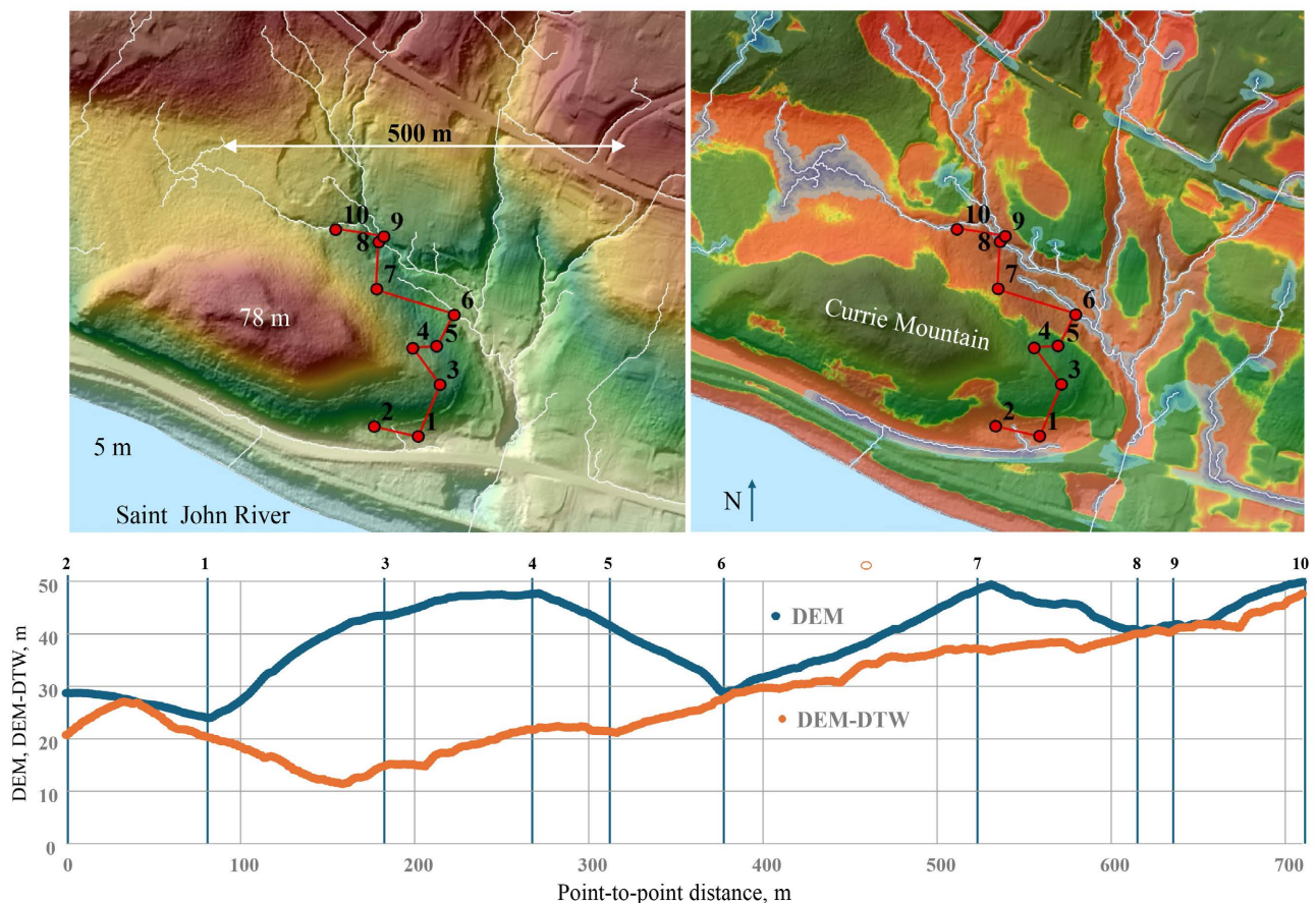
Figure 8. Hillshaded DEM (top left) and corresponding P_{rut}(y) projection regarding potential rut (red) and no-rut (green) occurrences (top right), overlaid by the DEM-derived FA > 1 ha flow channels, and the associated blue-shaded DTW_{FA>1ha} < 1 m layer. Also shown: 1) red dots numbered 1 to 10 referring to individually dug soil pits, done to assess the depths of mottle appearances as location-specific soil drainage indicators; 2) the corresponding point-to-point DEM and DEM-DTW elevation profiles (bottom). Location: 66.753W, 45.983N.
