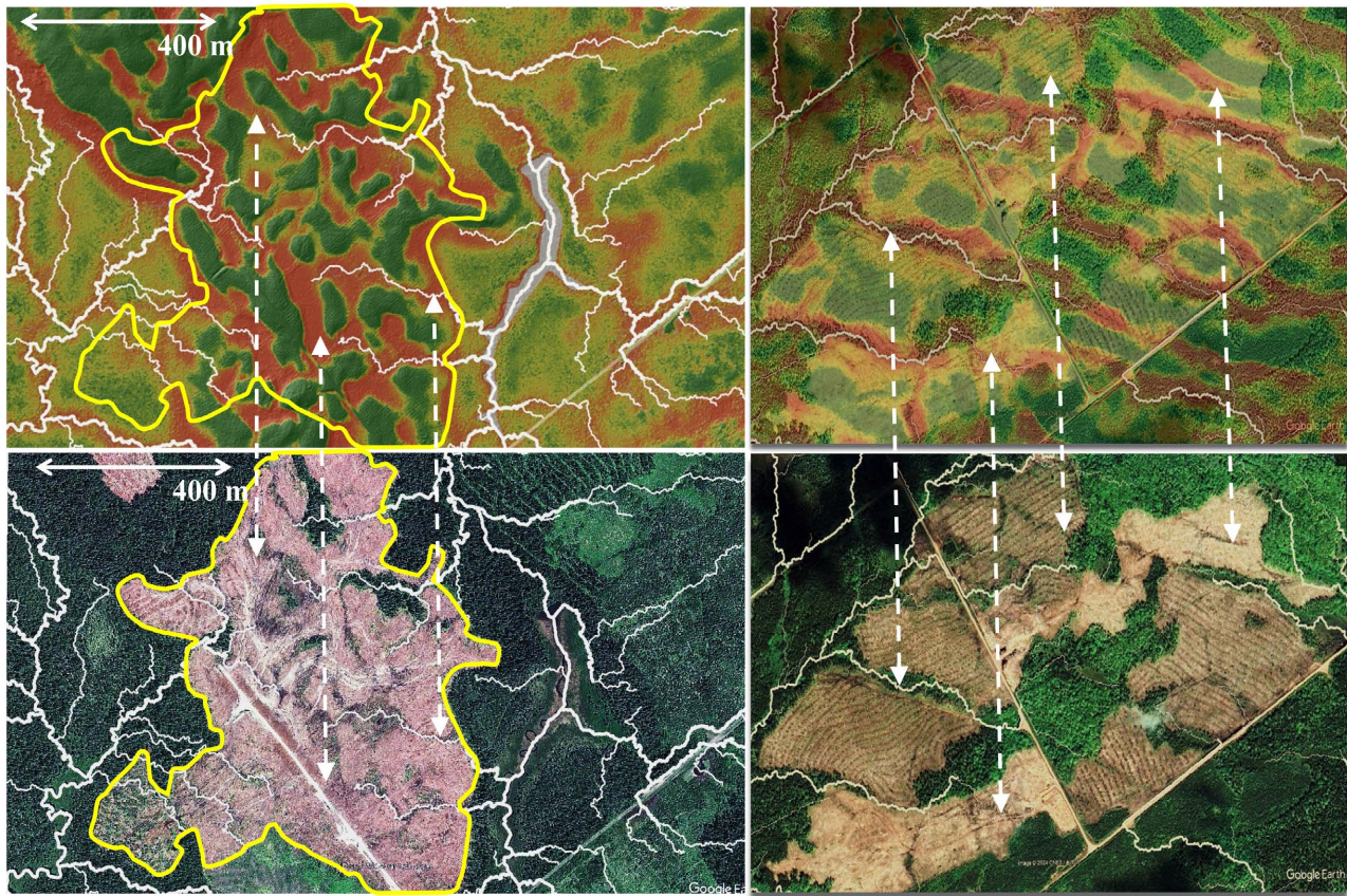
Figure 9. P_{\text{rut}}(y) projected rut occurrence zones (top) across a gently sloped (left) and a highly irregular (right) terrain in comparison with the corresponding Google Earth images (bottom). Example on the left: 46.195N, 65.780W; Google Earth Image June 2019. Example on the right: 47.322N, 67.755W; Google Earth Image June 2010. White lines: DEM-delineated stream channels with >1 ha FA (thin) and >4 ha FA (thick). Stippled lines: one-on-one correspondence guides.
