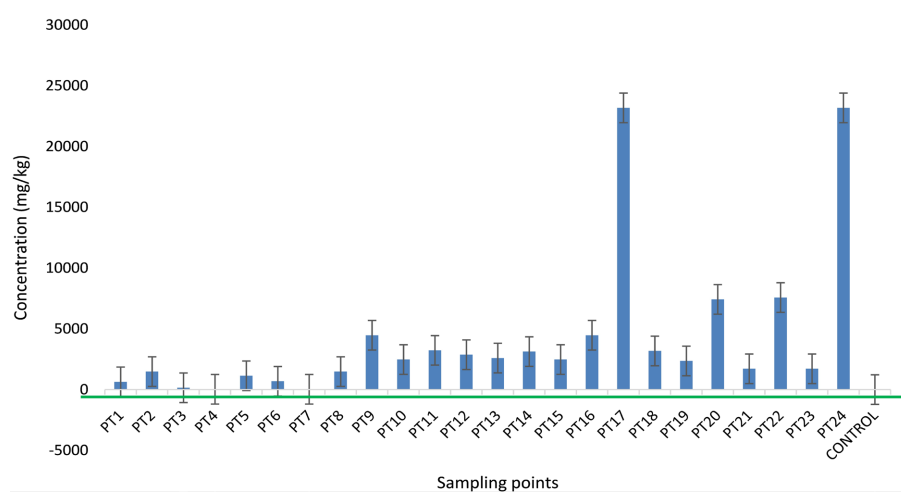
Figure 5. Concentration of Cu in crude oil-polluted soil in Okpare-Olomu community.
