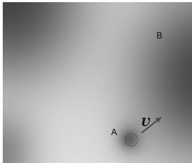
Figure 1. Our inhomogeneous infinite universe and the undefinability of an absolute reference system. Imagine an observable sector of the infinite universe (the solid line circle that indicates the sphere in which the observer is on the center) embedded in a high-density zone A of normal ordinary matter of mass about m . The observer's high-density region is attracted and accelerated by gravitation with an average velocity v towards a near region B of high density, higher mass M ( M \gg m ), and higher size. Region B is not observable from A and v cannot be known. All the observer's observable universe, his high-density region A, and many surrounding lower density regions are accelerated towards the Huge-Attractor B. CMB radiation is a material wave process propagating on the EM fields of the matter in region A, so it will not show any effect due to the movement of the matter of the whole region A towards the B one.
