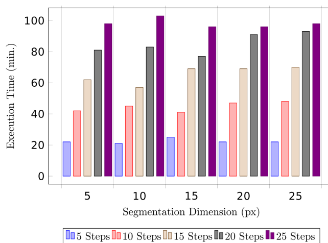
Figure 3. Scalability of the proposed algorithm on EMR with 2 data nodes.
