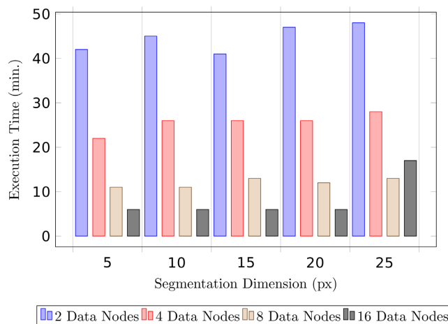
Figure 4. Scalability of the proposed ACO with a segmentation step of 10.
