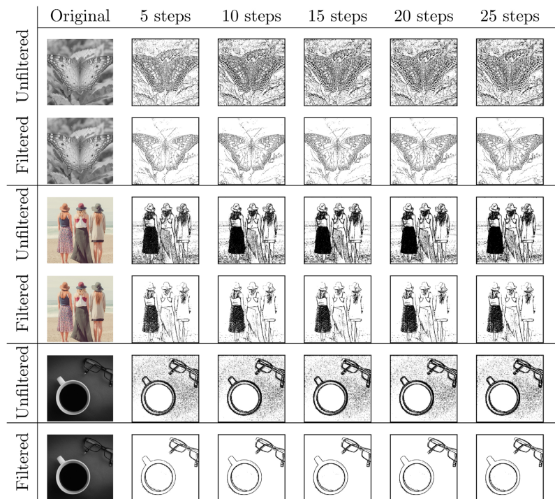
Figure 1. Detection results using unfiltered ACO and filtered ACO.
