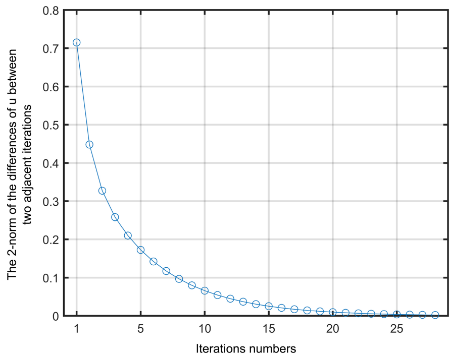
Figure 1. The 2-norm of the differences of u between two adjacent iterations from sonar dataset class 1.
