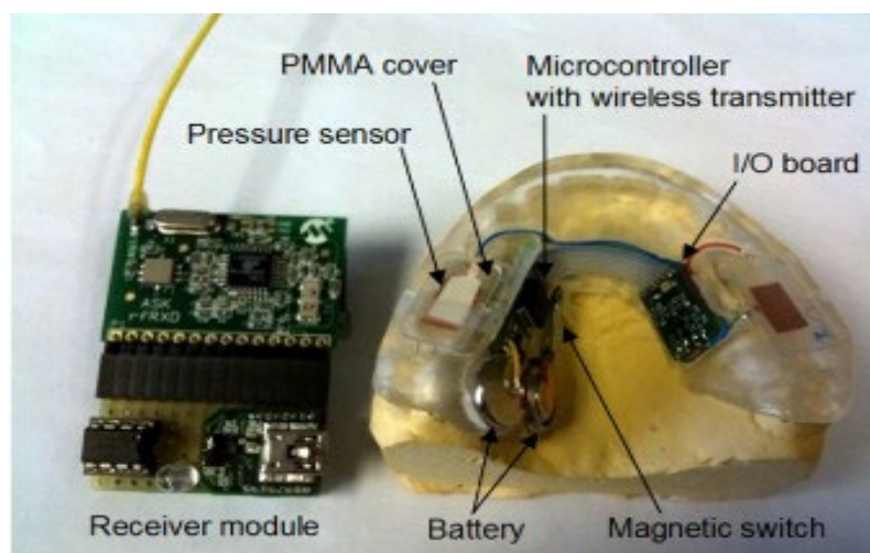
Figure 4. A wireless pressure sensing bite-guard has been developed for monitoring the progress of bruxism (teeth grinding during sleep); as well as protecting the teeth from damages [22].
