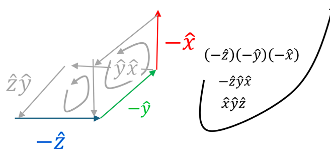
Figure 8. It is Figure 7 rotated by \hat{x} axis 180^\circ .
