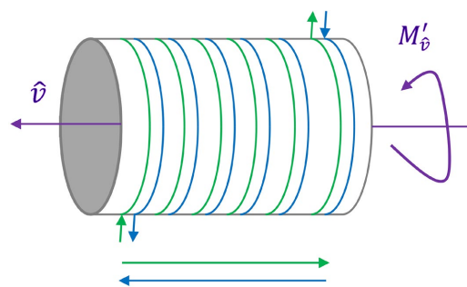
Figure 22. Creating a trivector in a coil. The green and blue cables in reality are twisted (represented parallel—instead of twisted—in the figure for simplicity). And the current will go in opposite direction in green and blue cables.
