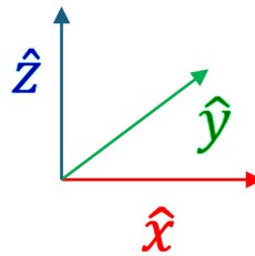
Figure 1. Basis vectors in three-dimensional space.
