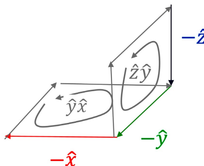
Figure 17. Trivector (-\hat{z})(-\hat{y})(-\hat{x}) .
