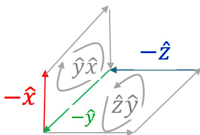
Figure 18. Trivector (-\hat{z})(-\hat{y})(-\hat{x}) .
