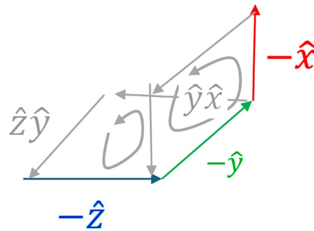
Figure 19. Trivector (-\hat{z})(-\hat{y})(-\hat{x}) .
