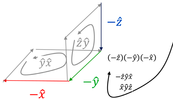
Figure 16. Trivector (-\hat{z})(-\hat{y})(-\hat{x}) = \hat{x}\hat{y}\hat{z} .
