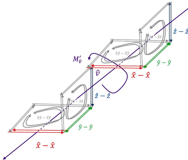
Figure 21. Adding consecutive trivectors.
