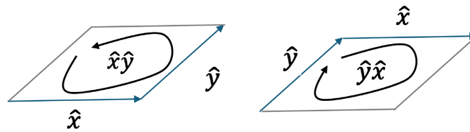
Figure 2. Representation of the bivectors \hat{x}\hat{y} and \hat{y}\hat{x} . They represent the same plane with opposite orientation. In fact, \hat{x}\hat{y} = -\hat{y}\hat{x} .
