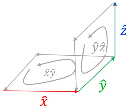
Figure 20. Trivector \hat{x}\hat{y}\hat{z} .
