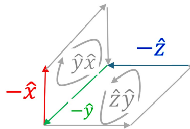
Figure 7. It is the same as Figure 6 rotated by \hat{y} axis clockwise.
