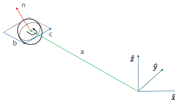
Figure 4. Representation position multivector.
