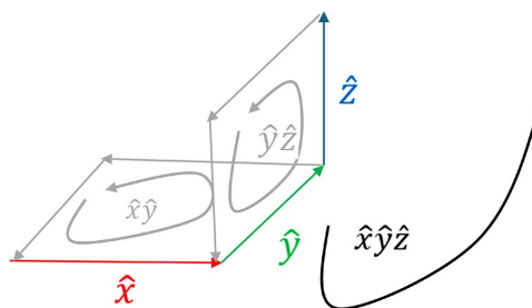
Figure 15. Trivector \hat{x}\hat{y}\hat{z} .
