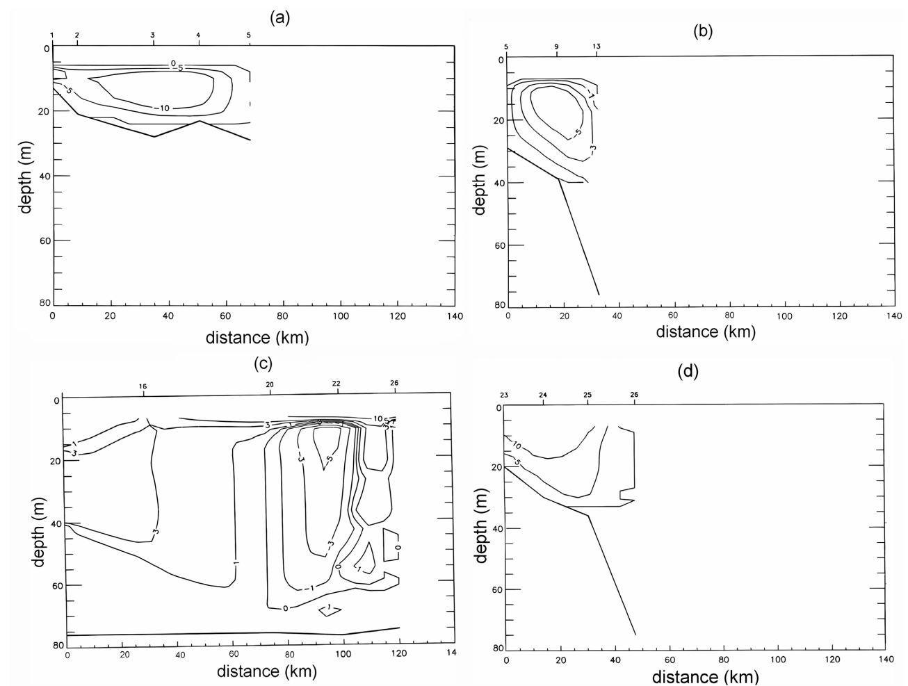
Figure 8. Cumulative salt flux contours into and out of the control volume using the 3 hour low passed mooring data over the period 15-19 February 1996: (a) through Side 1; (b) through Side 2; (c) through Side 3; and (d) through Side 4. Refer to text for details.
