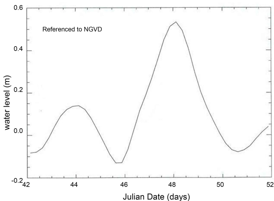
Figure 3. Water level at the NOAA NOS Duck, NC site over the period 11-21, February 1996. Raw data has been filtered as described below and then sub-sampled hourly to eliminate sub-inertial frequency motions to represent the storm induced time dependent coastal Ekman transport which resulted in a rise of 51 cm at the coast.
