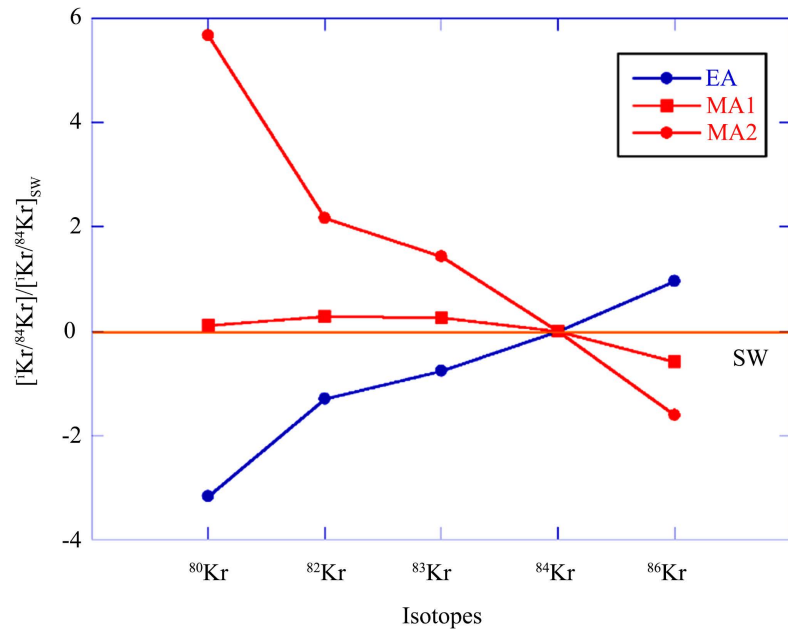
Figure 12. Krypton isotopes measured in different samples from glass inclusions in EETA 79001 showing MA2 (Mars atmosphere 1 (modern) with evidence of ^{80}\text{Kr} and ^{82}\text{Kr} excesses over the EA (Earth atmosphere) relative abundances.
