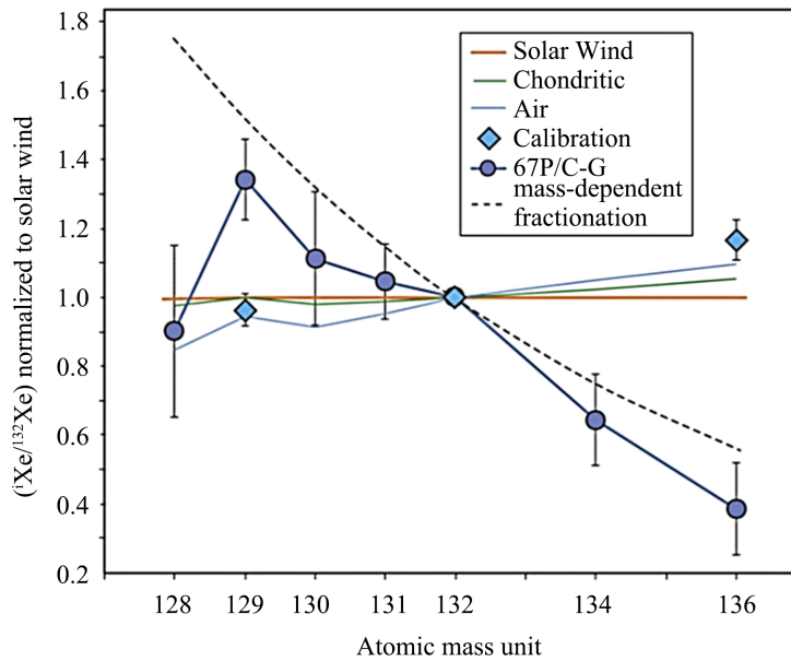
Figure 9. Xenon isotopic compositions of the Solar Wind, Earth’s Atmosphere, average Chondrite and primordial Comet ^{67}\text{P} . Figure taken from [25].
