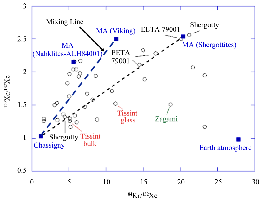
Figure 10. ^{129}\text{Xe} in Mars meteorites versus fission product Kr 84, both normed to ^{132}\text{Xe} showing an evolution of Mars environment from “primordial” Chassigny at 1.5 Gyr old to younger rock samples at 0.2 Gyr old and finally the modern Mars atmosphere. This shows an addition of a fission component to the Mars environment after its formation. Graph adapted from [1].
