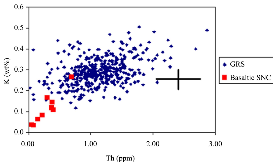
Figure 16. K, Th variations on Mars compared to Mars Meteorites (SNC). Typical Uncertainty is shown on the right. Figure taken from [42]. For comparison K is 2% wt. and Th 6 ppm of Earth's crust.
