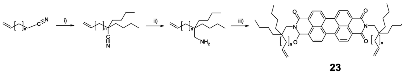
Figure 3. Synthesis of the starting materials for metathesis: 23 , n = 1 until 3 by means of alkylation of terminal alkenyl nitriles, reduction and condensation. i) C_4H_9I , LDA; ii) LiAlH_4 ; iii) Perylene-3,4:9,10-tetracarboxylicbisahydride, zinc acetate, imidazole.
