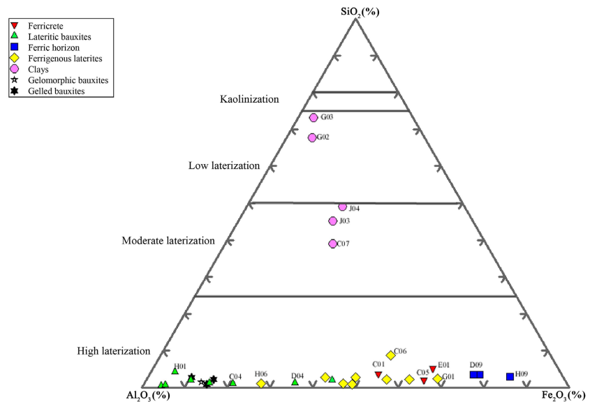
Figure 8. Triangular diagram between Al_2O_3 - Fe_2O_3 - SiO_2 (Schellmann, 1986).
