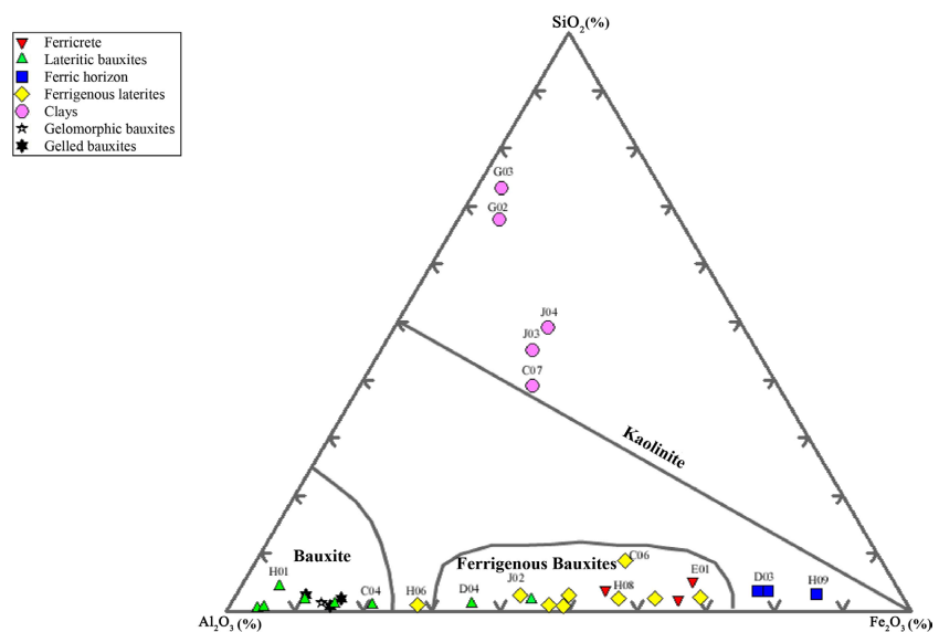
Figure 9. Triangular diagram between Al_2O_3 - Fe_2O_3 - SiO_2 (Boulangé et al., 1996).
