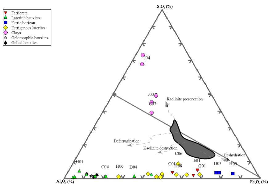
Figure 10. Triangular diagram between \text{Al}_2\text{O}_3 - \text{Fe}_2\text{O}_3 - \text{SiO}_2 from (Tardy, 1997).
