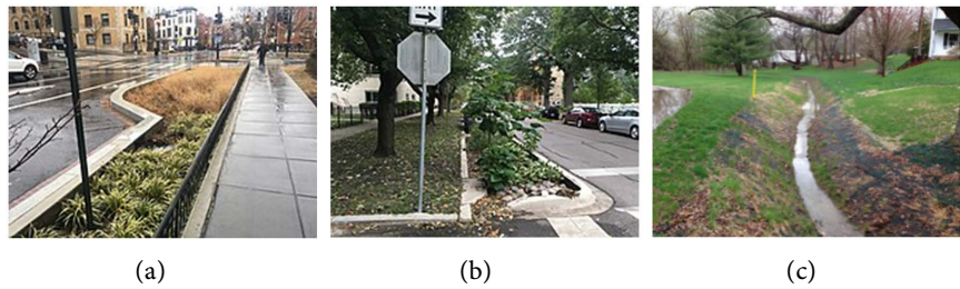
Figure 6. (a) Runoff from the vicinity flows into an adjacent bioswale; (b) Swale drain.
