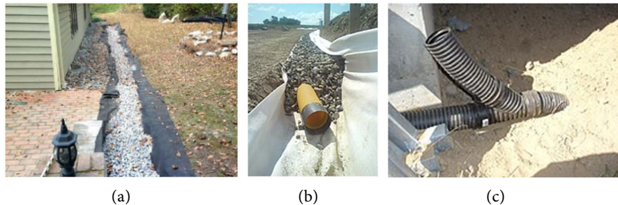
Figure 3. (a), (b) French drain under construction; (c) A wye-joining a perforated and solid corrugated pipe to a buried solid outlet.
