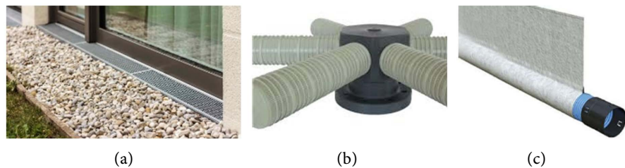
Figure 4. (a) Curtain drain; (b) Collector drain; (c) Fin drain.
