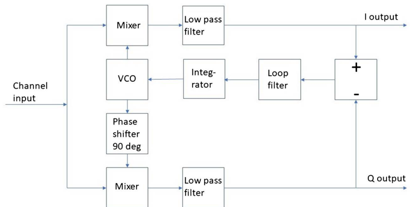
Figure 1. Costas loop for 4QAM demodulation.
