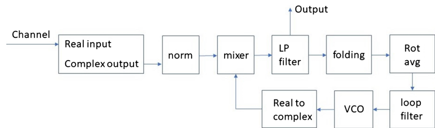
Figure 11. Block diagram of the improved Masterpiece.
