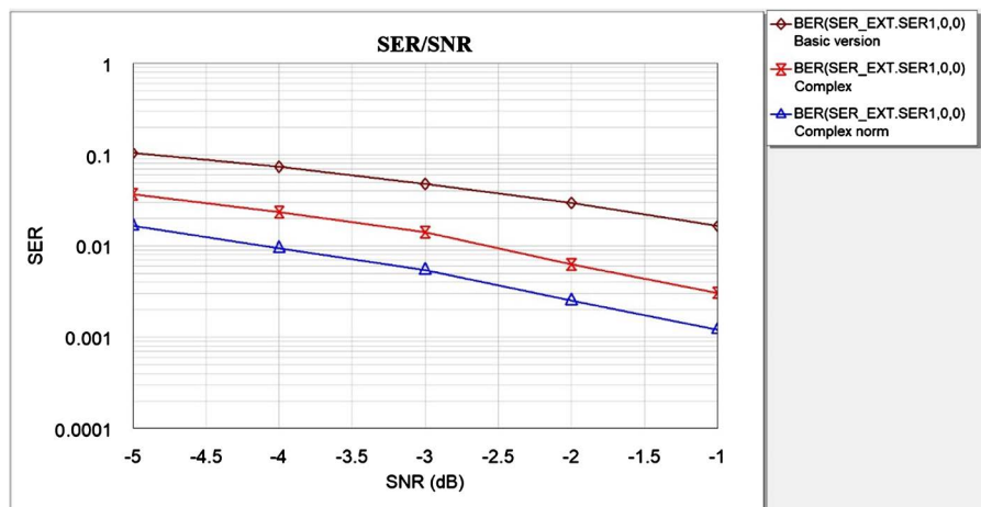
Figure 4. Effect of application of a complex signal and its normalization on noise properties. Three curves for SER vs. SNR are shown. The upper curve is without complex signal. The middle curve is with complex signal but without normalization. Bottom curve is with normalization.
