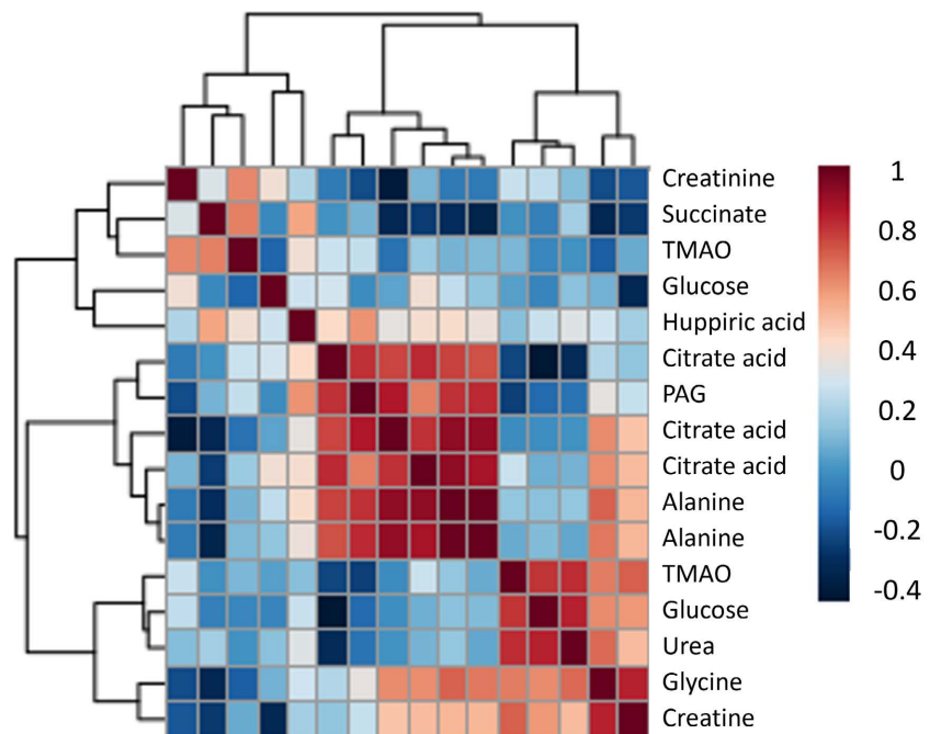
Figure 4. Note the correlation heatmaps will only show correlations for a maximum of 1000 features. For larger datasets, only the top 1000 features will be selected based on their interquartile range (IQR). When the color distribution is fixed, you can potentially compare the correlation patterns among different data sets.
