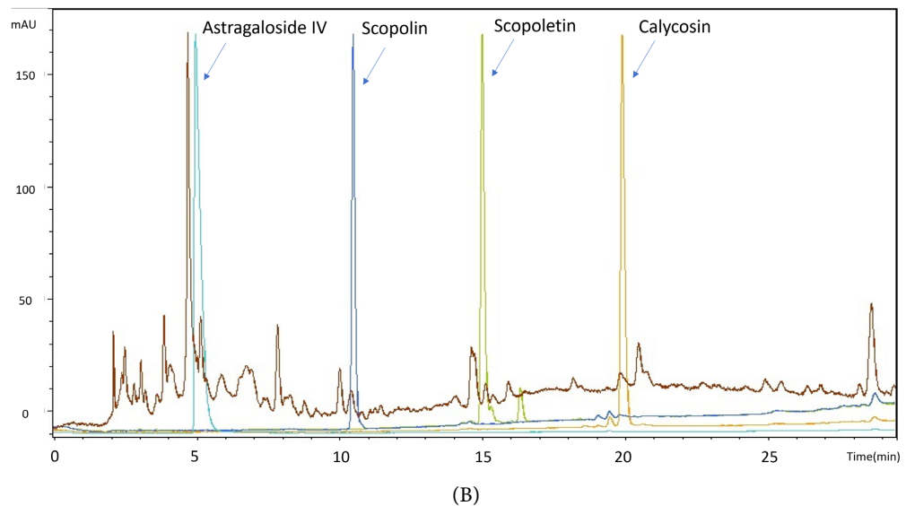
Figure 11. (A) The TCM tea analysis by LC-MS. (B) Overlay comparison of sample analysis chart and four standard products.
