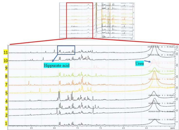
Figure A1. The spectrum of urine analyzed by NMR.
