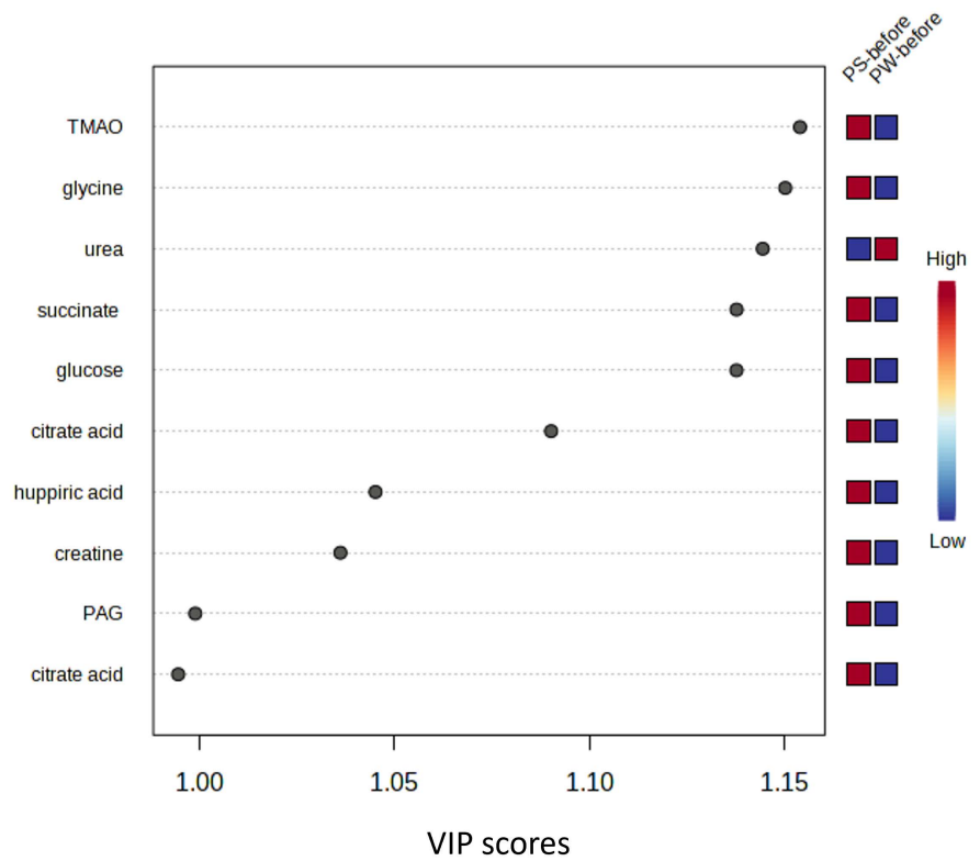
Figure 3. Variable importance in projection (VIP) score plot for the top 10 most important metabolite features.
