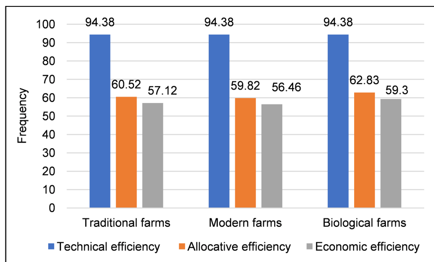
Figure 2. Distribution of efficiency scores by farm groups.
