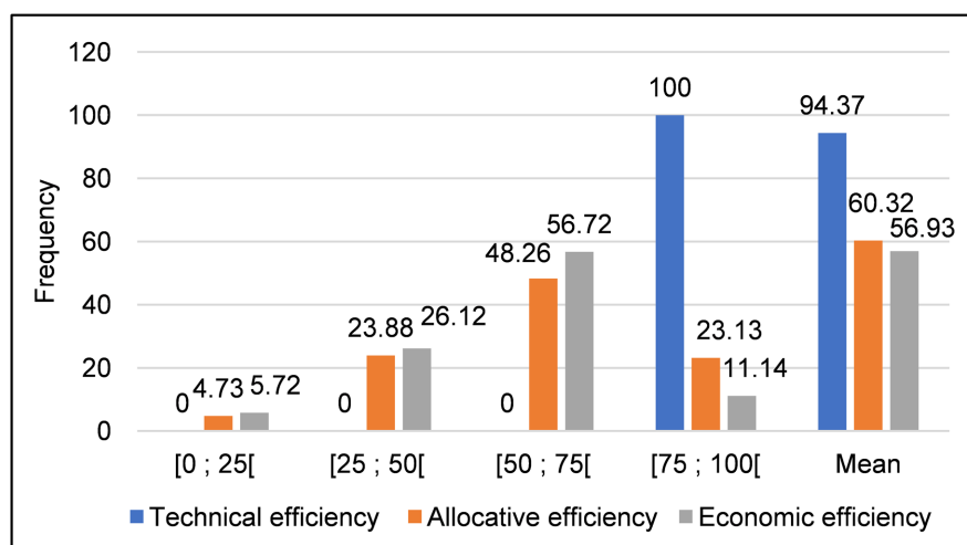
Figure 1. Producer frequencies by type of technical, allocative and economic efficiency.
