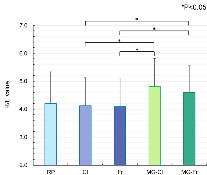
Figure 3. Results of multiple comparison test on differences in R/E value due to occlusal conditions. Measurements are expressed as means + SD. Error bar indicates standard error of the mean. * P < 0.05 ; denotes statistically significant difference.
