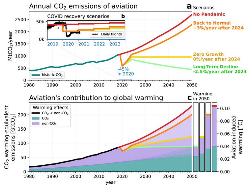
Figure 1. Aviation's contribution to global warming till 2050. (a) Annual historic and future annual carbon dioxide (CO 2 ) emissions of aviation following four scenarios: No pandemic, back to normal, zero long-term growth, and long-term decline. (b) Daily flights of selected airports globally between 2019 and November 2020 and annual averages for all scenarios. (c) Cumulative warming-equivalent emissions of CO 2 and non-CO 2 effects of aviation since 1940 and the corresponding aviation-induced global warming. Scenarios are color-coded as in (a) [5].
