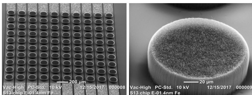
Figure 4. Electron microscope images showing patterned nanotubes that would operate as an electron emitter in a new instrument now being developed for analyzing extraterrestrial samples. The right image is a close-up of one of the bumps. To create these highly versatile structures, technicians place a silicon wafer or some other substrate inside a furnace. As the oven heats, they bathe the substrate with a carbon feedstock gas to produce the thin coating of nearly invisible hair-like structures. Credits: NASA [18].
