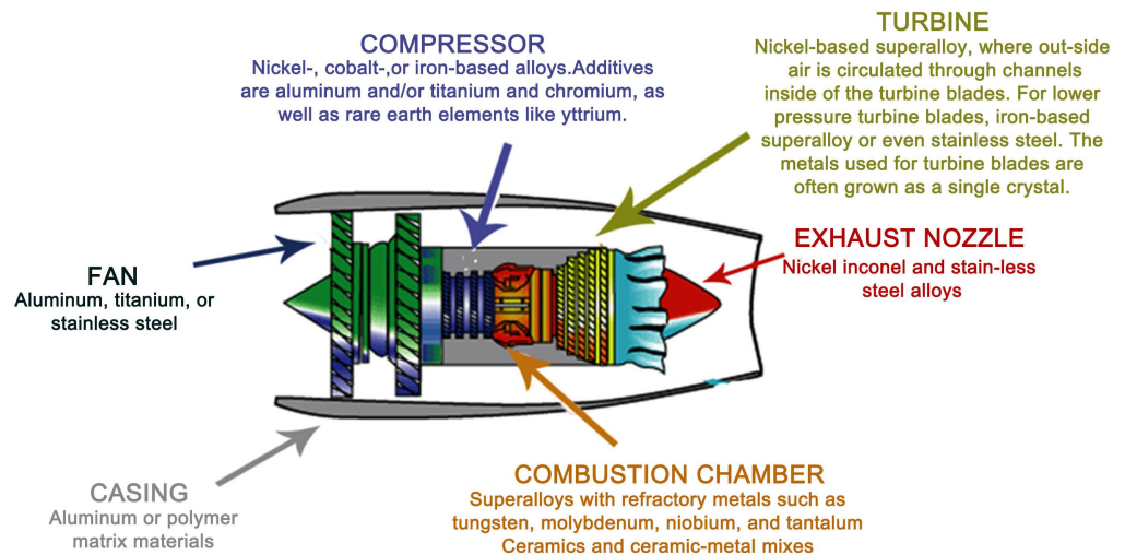
Figure 2. Proposed composite materials of a jet engine and areas of nanotechnological incorporation to reduce the impact on the environment. Reprinted with permission of the “PreScouter” [9] [10].
