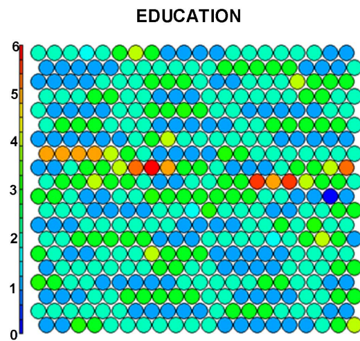
Figure 4. Data distribution by education.
