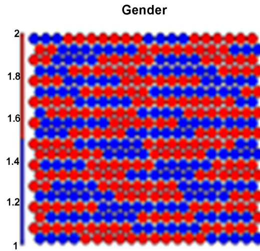
Figure 2. Data distribution by gender.
