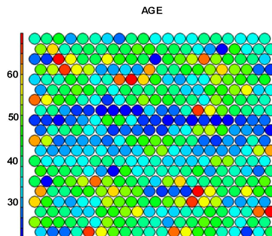
Figure 1. Data distribution by age.
