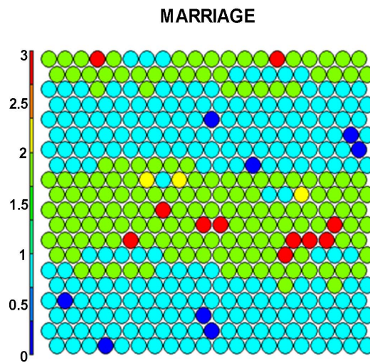
Figure 3. Data distribution by marriage.
