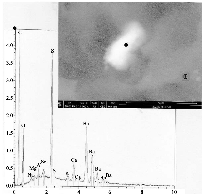
Figure 26. A first example of a barytine particle on hair number 1. Above: SEM photograph (in CBS, 12,000 \times ) of the barytine particle, located on a portion of hair number 1. Below: spectrum at the black dot. C: carbon; O: oxygen; Na: sodium; Mg: magnesium; Al: aluminium; Sr: strontium; S (two peaks): sulphur; K: potassium; Ca (two peaks): calcium; Ba (five peaks): barium.
