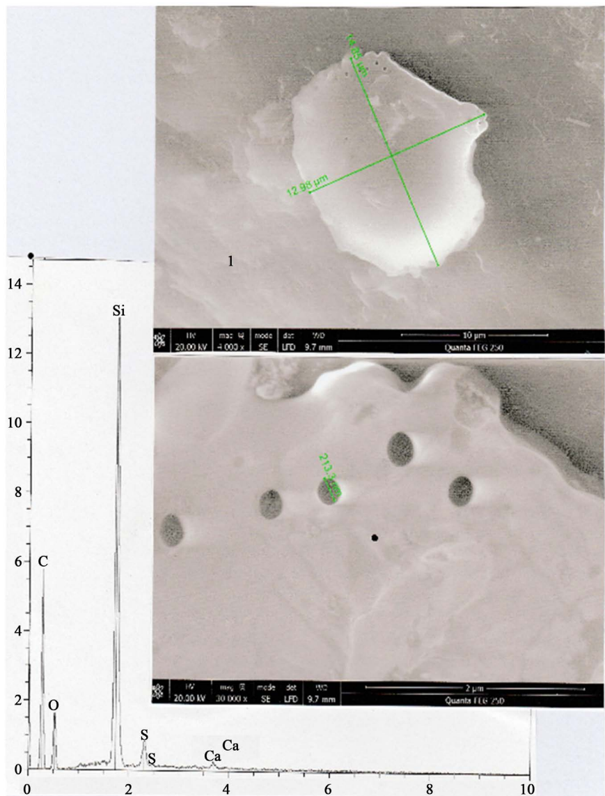
Figure 8. The second diatom observed, on hair number 1. Upper photograph: SEM photograph (in LFD, 4000×) showing this broken diatom on hair 1 portion. Lower photograph: enlarged photograph (30,000×) showing the diatom pores. Below: spectrum at the little black dot.
