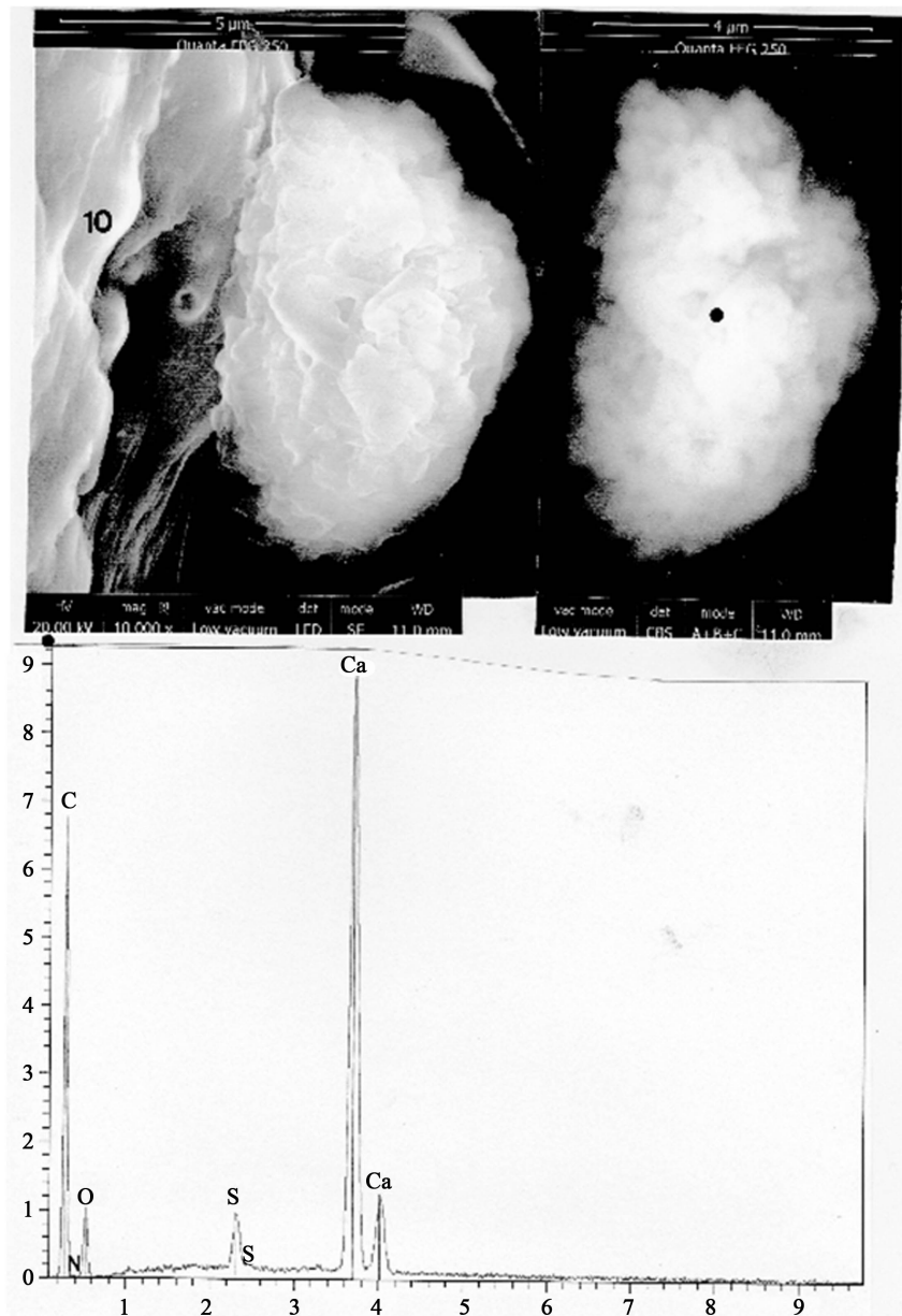
Figure 11. One coccolith located near the hair number 10. Above: SEM photographs (in LFD at the left, and in CBS at the right) 10,000× of the coccolith, located at the proximity of a portion of the hair number 10. Below: spectrum at the little black dot. C: carbon; N (traces): nitrogen; O: oxygen; S (two peaks): sulphur; Ca (two peaks): calcium.
