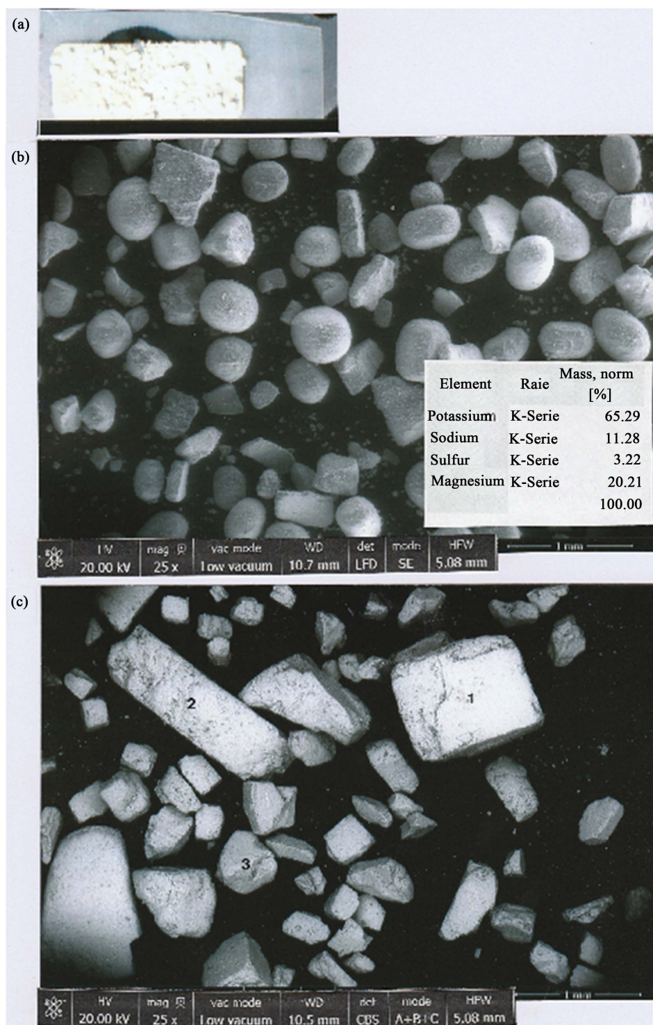
Figure S1. Study of a light salt powder. (a): optical view (2x) of the powder; (b): SEM photograph (in LFD, 25x) of a sample of the powder. Insert: normalized (chlorine excepted) composition of the powder. C: SEM photograph (in CBS, 25x) of another sample of the powder. 1: a sodium chloride (ClNa) crystal; 2: a potassium chloride (KCl) crystal; 3: a magnesium chloride (MgCl 2 ) crystal.
