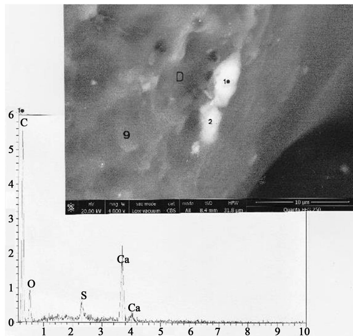
Figure 10. Another diatom (observed by pores only) on hair number 9. Above: SEM photograph (in CBS, 4000×) of the diatom (D), located at some part of hair number 9 (1 and 2 are two adjacent particles located near the diatom). Below: spectrum (in 1) at the little black dot. C: carbon; O: oxygen; S: sulphur; Ca (two peaks): calcium.
