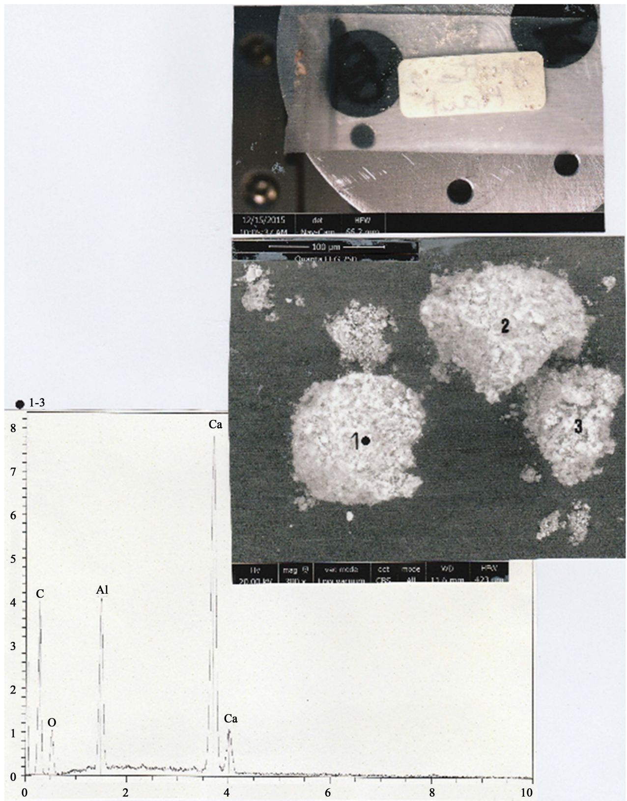
Figure S4. Study of the coating of the ceiling of the cave. Above: optical view (2×) of the coating powder. Below: SEM photograph (in CBS, 300×) of three (1 - 3) well separated aggregates of the coating. Spectrum (at the black dot), that is common to 1 - 3. C: carbon; O: oxygen; Al: aluminium; Ca (two peaks): calcium.
