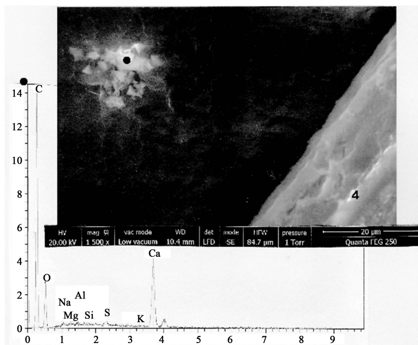
Figure 15. A tintinnid located near the hair number 4. Above: SEM photograph (in LFD, 1500×) of the tintinnid specimen, near a portion of hair number 4. Below: spectrum at the black dot. C: carbon; O: oxygen; Na: sodium; Mg: magnesium; Al (traces): aluminium; Si (traces): silicium; S: sulphur; K (traces): potassium; Ca (two peaks): calcium.
