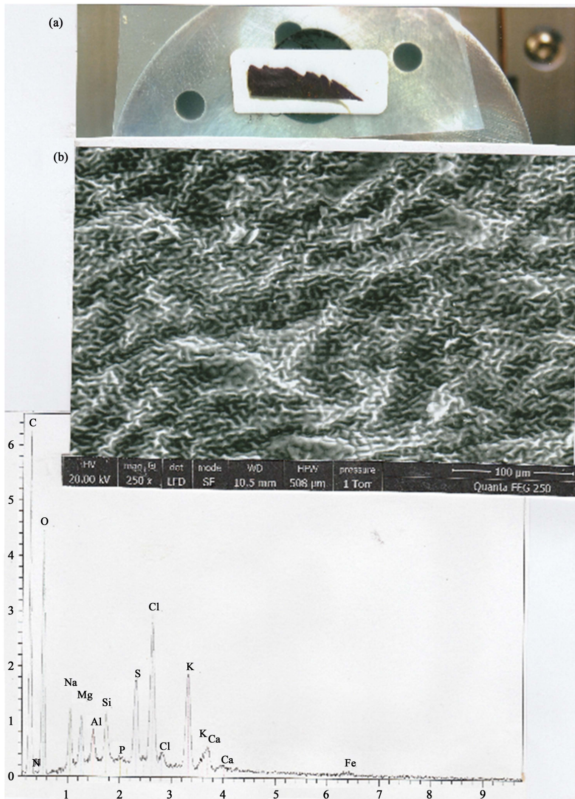
Figure S2. Study of a thalle of Fucus . (a): optical view (2×) of a surface portion of the Fucus ; (b): SEM photograph (in LFD, 250×) of the surface portion; (c): global spectrum of the surface. C: carbon; N: nitrogen; O: oxygen; Na: sodium; Mg: magnesium; Al: aluminium; Si: silicium; P: phosphorous; S (two peaks): sulphur; K (two peaks): potassium; Ca (two peaks): calcium; Fe (traces): iron.
