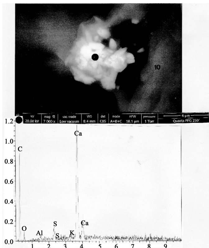
Figure 17. A third tintinnid located on the hair number 10. Above: SEM photograph (in CBS, 7000×) of the tintinnid specimen, on a portion of hair number 10. Below: specimen at the black dot. C: carbon; O: oxygen; Al: aluminium; S (two peaks): sulphur; K (traces): potassium; Ca (two peaks): calcium.
