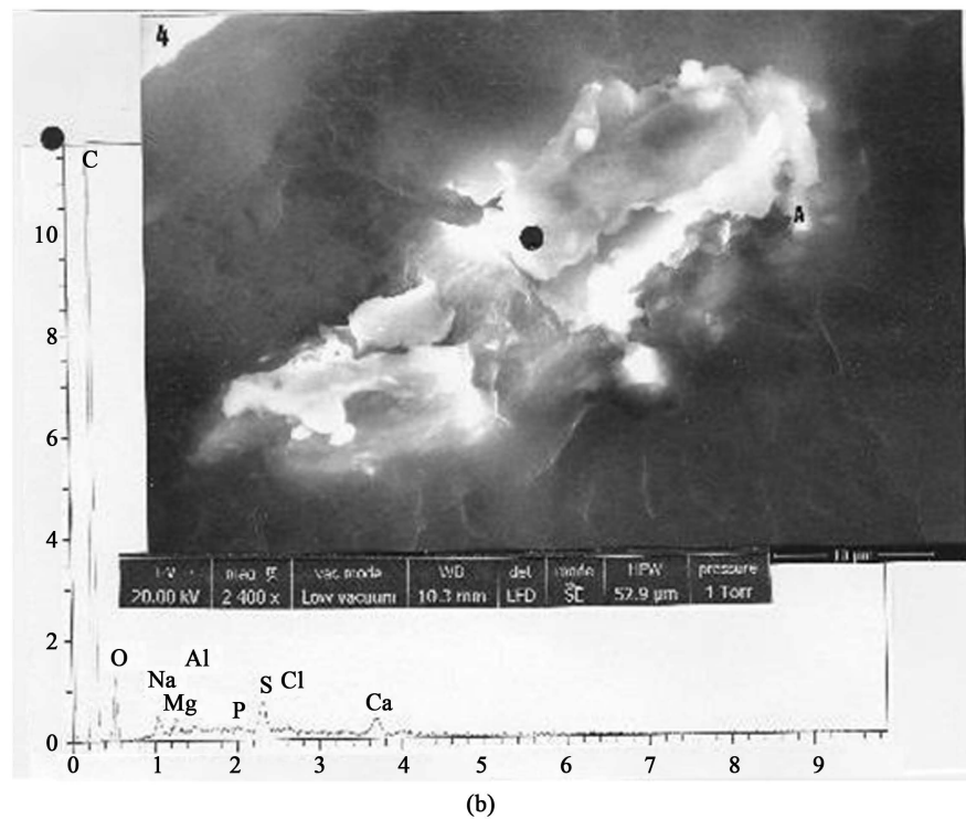
Figure 23. Crustacean shell sheets on hair number 9 and at the vicinity of hair number 4. A: shell sheets on some part of hair number 9. Above: SEM photograph (in CBS, 4 000×) of the shell sheets. PL: the sheets; A: appendages. Below: spectrum at the black dot. B: shell sheets at the vicinity of hair number 4 (A: appendage). Above: SEM photograph (in LFD, 2400×) of the shell sheets. Below: spectrum at the black dot.
