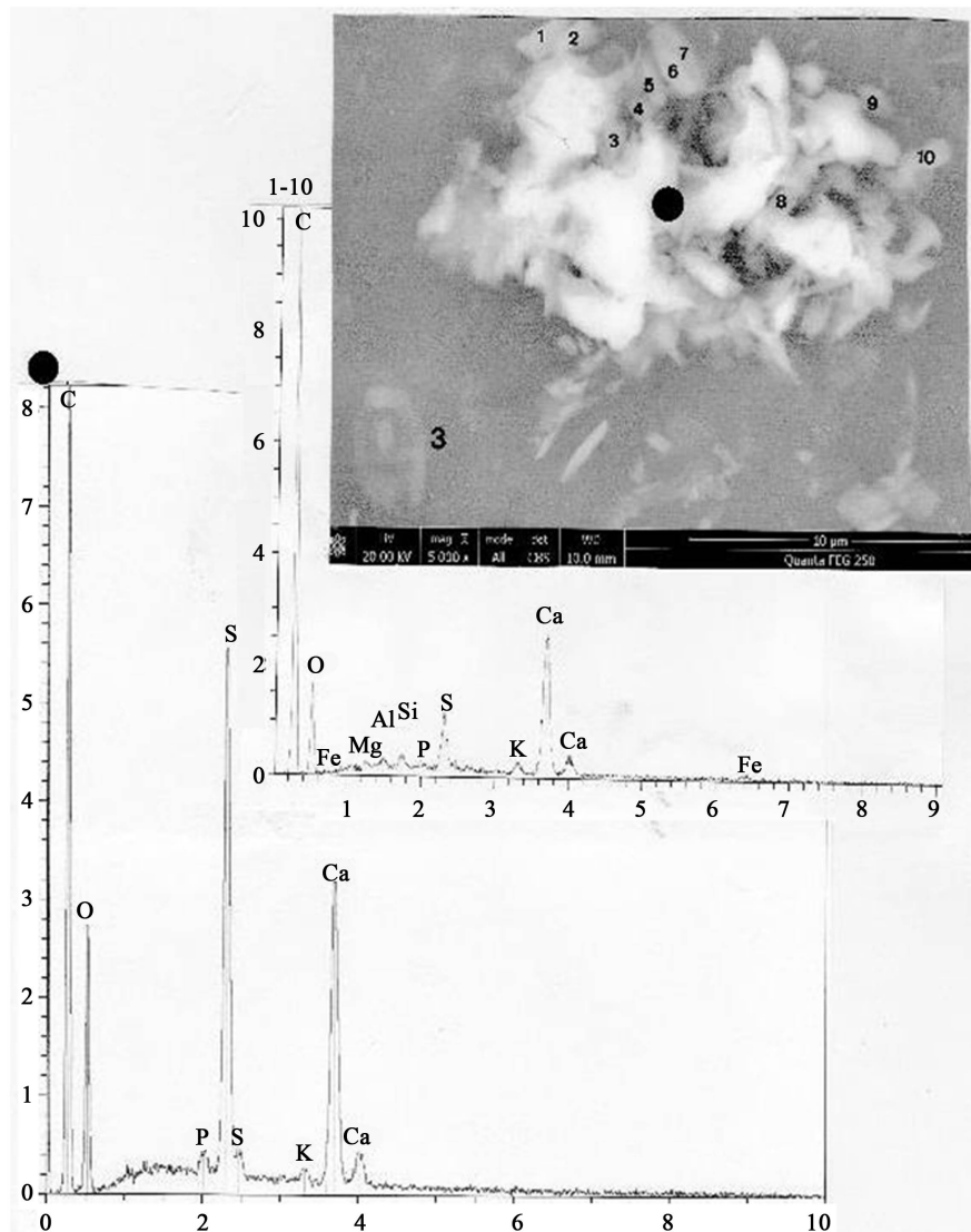
Figure 4. Gypsum and aragonite crystals on hair number 3. Above: SEM photograph (in CBS, 5000 \times ) of the pile of gypsum crystals located on another part of a hair number 3 portion (1 - 10: little mineral particles). Below: spectrum at the black dot; upper spectrum: 1 - 10 spectras.
