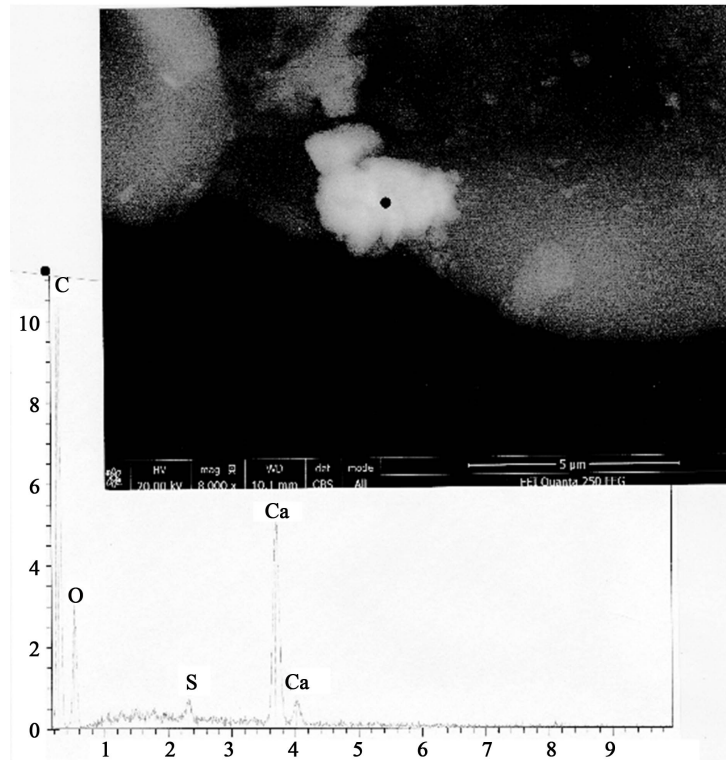
Figure 12. Above: SEM photograph (in CBS, 8000×) of another coccolith, located on a portion of hair number 2. Below: spectrum at the little black dot.
