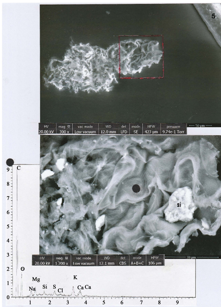
Figure 20. A third thalle of an algae located in the vicinity of hair number 5; upper photograph : (in LFD, 300×) of the thalle; the red rectangle area is enlarged in the below photograph. Lower photograph : SEM photograph (in CBS) of the enlarged (1200×) rectangle area; Si: a silica particle. Below : spectrum at the black dot. C: carbon; O: oxygen; Na: sodium; Mg: magnesium; Si: silicium; Cl: chlorine; K: potassium; Ca (two peaks): calcium.
