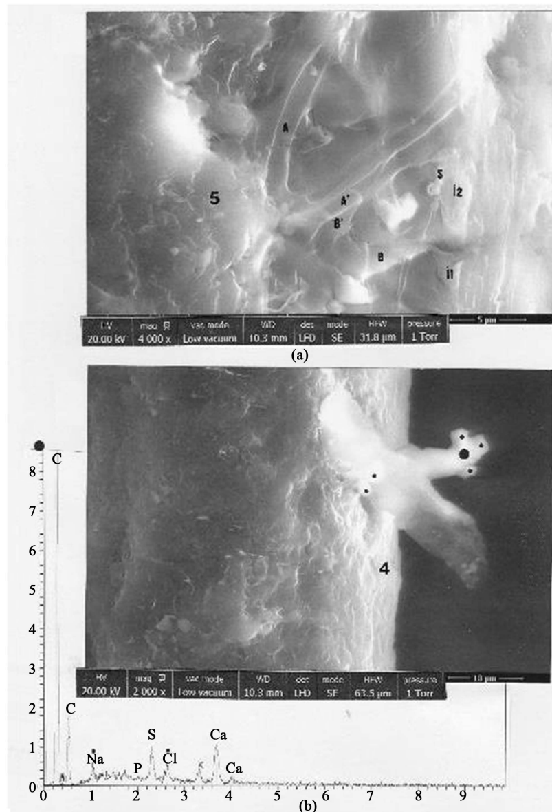
Figure 22. Crustacean appendages on hair number 4 and 5. Upper (A) photograph: SEM photograph (in LFD, 4000 \times ) of some portions of binamous appendages located on some part of hair number 5. AA' and BB': the two parts of two biramous appendages A and B; i1 and i2: some portions of appendages; S: bristle of an appendage. Lower (B) photograph: SEM photograph (in LFD, 2000 \times ) of a biramous appendage portion located at the right border of some part of hair number 4; little points indicate particle of salt crystals. Below: spectrum at the black dot. C: carbon; N: nitrogen; O: oxygen; Na: sodium; P (traces): phosphorous; S: sulphur; Cl: chlorine; K: potassium; Ca (two peaks): calcium. Na and Cl elements are pointed.
