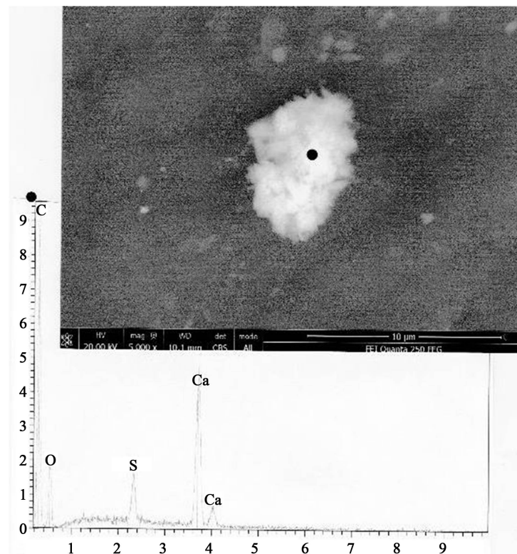
Figure 13. Above: SEM photograph (in CBS, 5000×) of a second coccolith located on another portion of hair number 2. Below: spectrum at the black dot.
