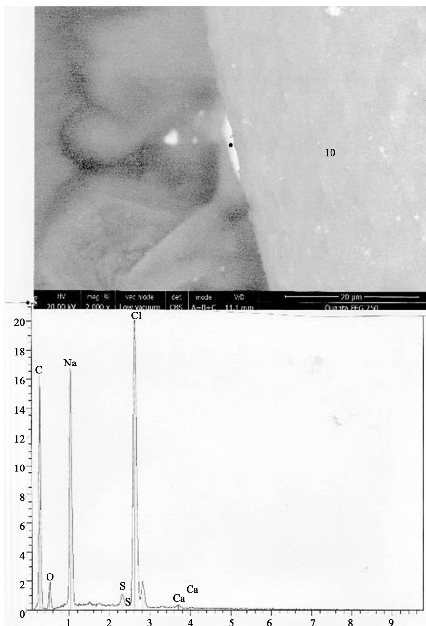
Figure 5. A salt powder on the hair number 10. Above: SEM photograph (in CBS, 2000×) showing the powder. Below: spectrum at the little black dot. C: carbon; O: oxygen; Na: sodium; S: sulphur; Cl (two peaks): chlorine; Ca: calcium.
