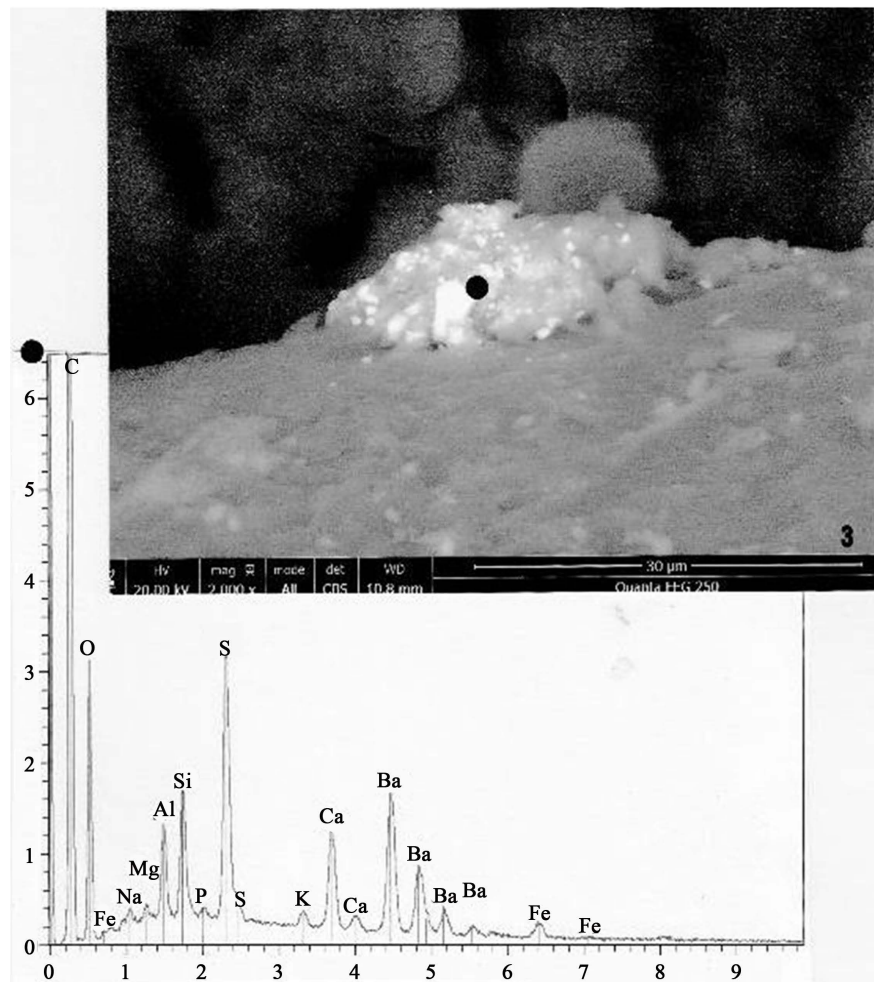
Figure 30. A micro-scale of barium sulphate pigment on hair number 3. Above: SEM photograph (in CBS, 2000×) of the micro-scale, located on some part of the hair number 3 surface. Below: spectrum at the black dot. C: carbon; O: oxygen; Fe (three peaks): iron; Na: sodium; Mg: magnesium; Al: aluminium; Si: silicium; P: phosphorous; S (two peaks): sulphur; K: potassium; Ca (two peaks): calcium; Ba (four peaks): barium.
