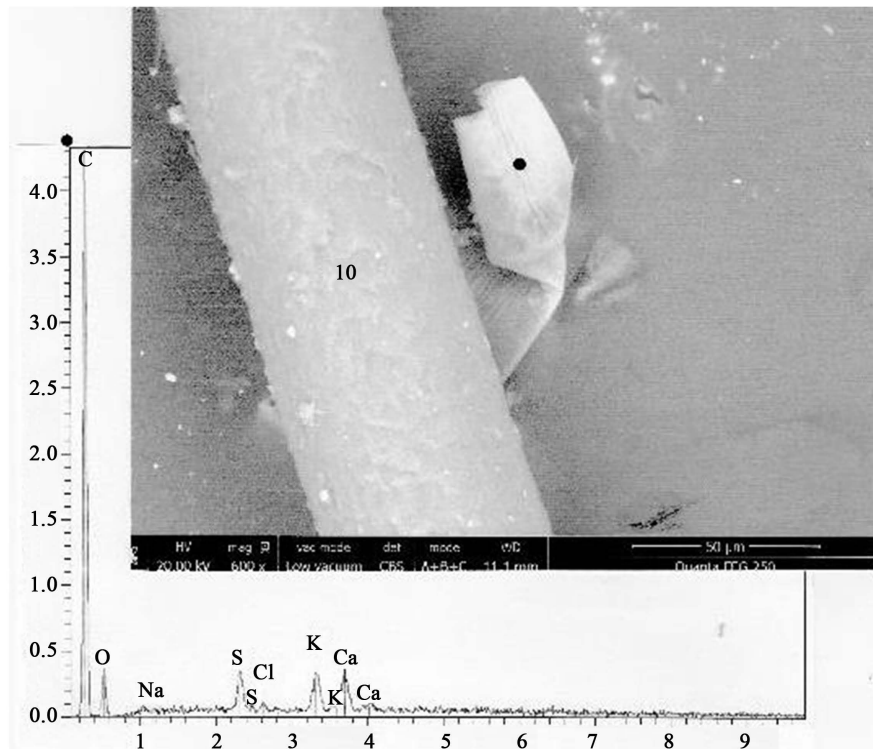
Figure 19. Another algae fragment on hair number 10. Above: SEM photograph (in CBS, 600×) of a thalle portion of the algae, surrounding some part of hair number 10. Below: spectrum at the little black dot. C: carbon; O: oxygen; Na: sodium; S (two peaks: sulphur); Cl: chlorine; K (two peaks): potassium; ca (two peaks): calcium.
