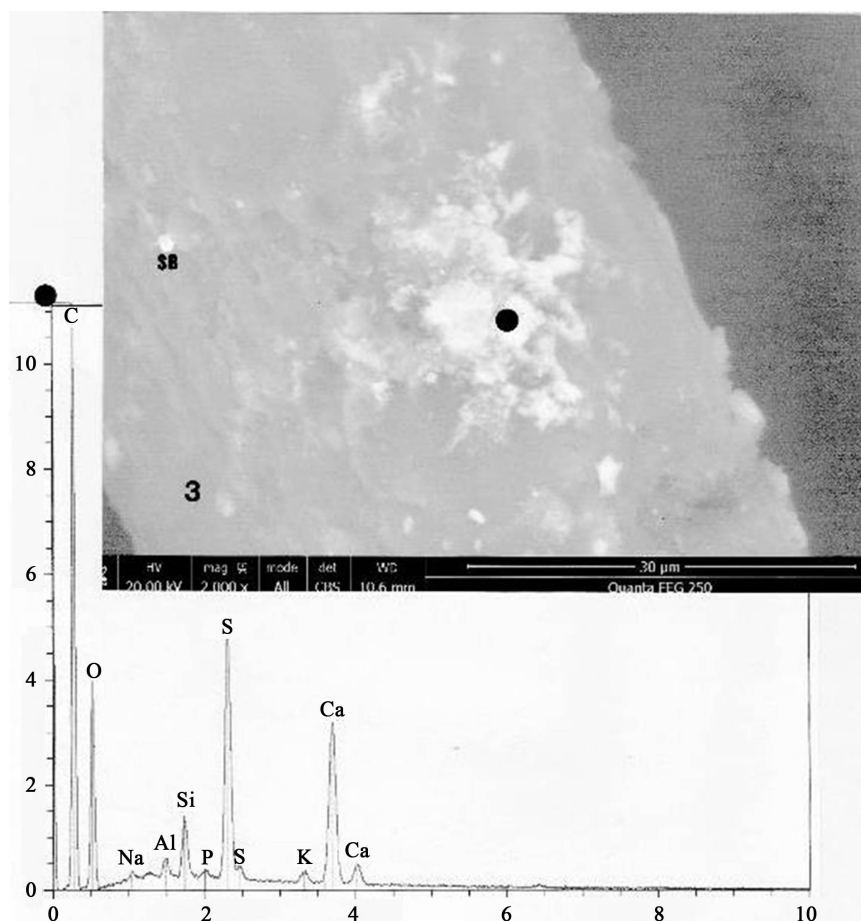
Figure 3. Gypsum pile on hair number 3. Above: SEM photograph (in CBS, 2000×) of a gypsum pile located on hair number 3 portion. The black dot indicates the location where EDX analysis is realized. (SB: a particle of barium sulphate). Below: spectrum at the black dot. C: carbon; O: oxygen; Na: sodium; Si: silicium; P: phosphorous; S (two peaks): sulphur; K: potassium; Ca (two peaks): calcium.
