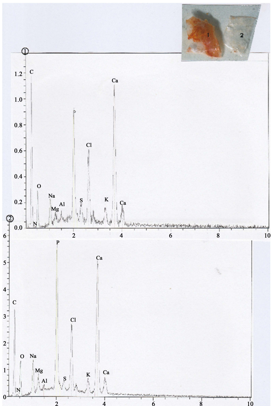
Figure S3. Study of a pawn shell. Above: optical view (2×) of the shell. 1: colored (red) shell fragment (dorsal); 2: white (ventral) shell fragment. Below: spectras of 1 and 2 . C: carbon; N (traces): nitrogen; O: oxygen; Na: sodium; Mg: magnesium; Al: aluminium; P: phosphorous; S: sulphur; Cl (two peaks): chlorine; K: potassium; Ca (two peaks): calcium.
