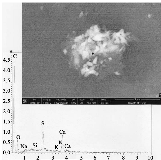
Figure 16. Another tintinnid located near the hair number 9. Above: SEM photograph (in CBS, 8000×) of the tintinnid specimen, near a portion of hair number 9. Below: spectrum at the little black point. C: carbon; Na: sodium; Si: silicium; S (two peaks): sulphur; K (traces): potassium; Ca (two peaks): calcium.
