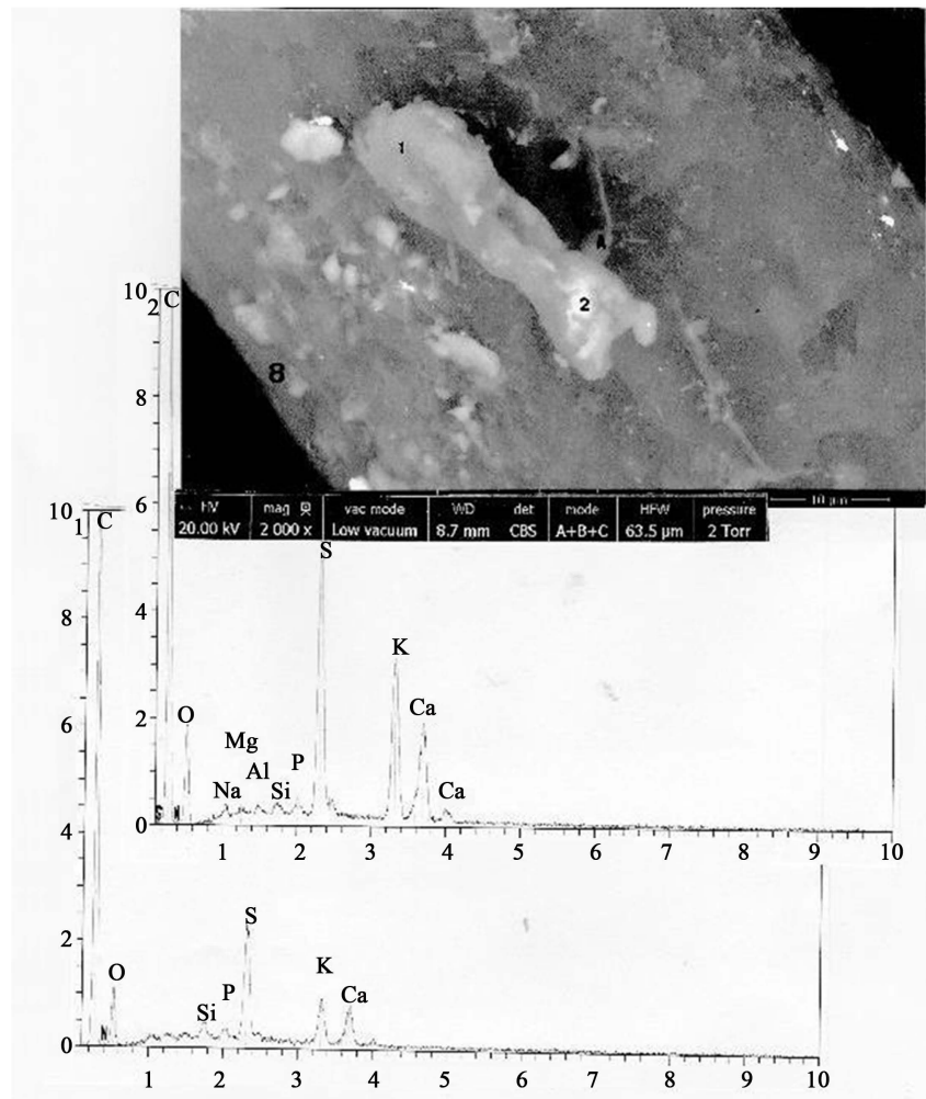
Figure 21. A shell portion of a crustacean on hair number 8 . Above : SEM photograph (in CBS, 2000×) of the shell portion, located on some part of hair number 8 (1: the smooth portion of the shell; 2: the granulous portion of the shell; A: an appendage). Below : lower spectrum: that of 1. Upper spectrum: that of 2. S (three peaks): sulphur; C: carbon; N: nitrogen; O: oxygen; Na: sodium; Mg: magnesium; Al: aluminium; Si: silicium; P: phosphorous; K: potassium; Ca (two peaks): calcium.
