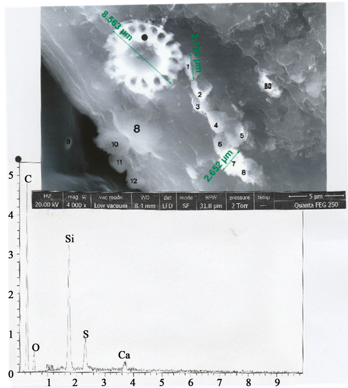
Figure 9. Two diatoms on an hair number 8 portion. Above: SEM photograph (in LFD) showing an enlarged (4000×) view of the rectangle area of Figure 1 . BD: broken part of another diatom; 1 - 12: modern spores. Below: spectrum at the black dot.
