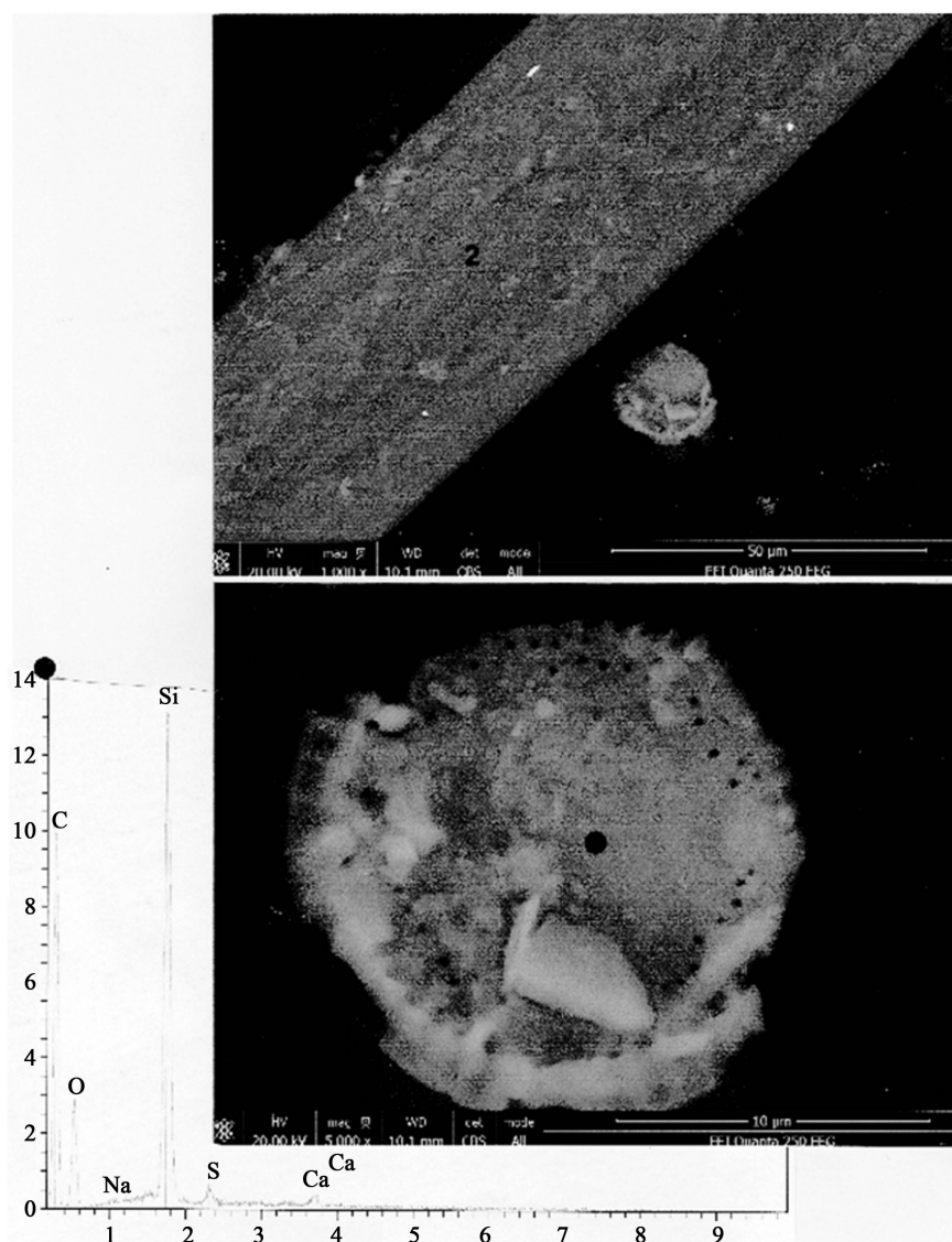
Figure 7. The first complete diatom observed, at the proximity of hair number 2. Upper photograph: SEM photograph (in CBS, 1000×) showing the diatom at the proximity of an hair 2 portion. Lower photograph: enlarged photograph (5000×) of the diatom. Below: spectrum at the black dot. C: carbon; O: oxygen; Na (traces): sodium; Si: silicium; S: sulphur; Ca: calcium.
