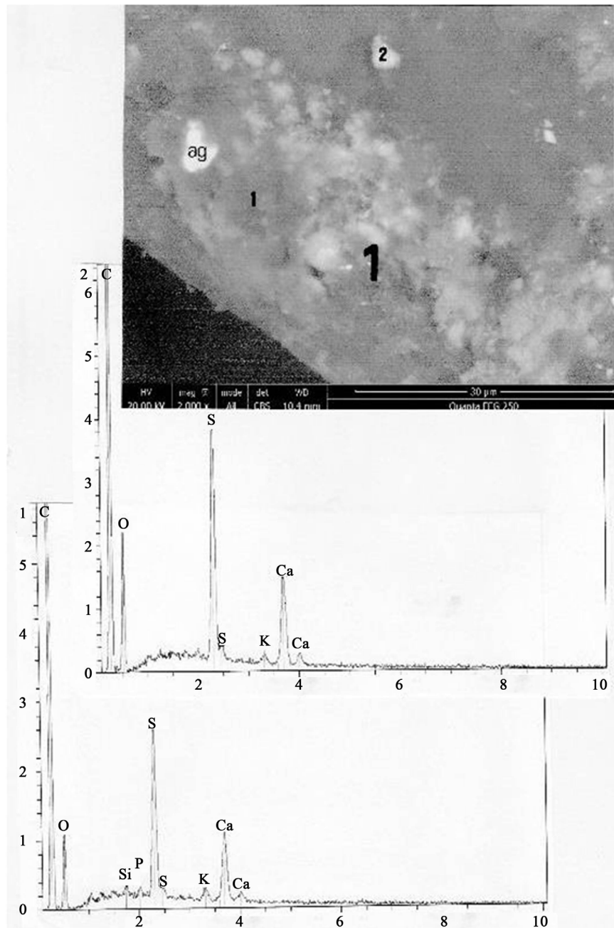
Figure 2. Calcium sulphate on hair number 1. Above: SEM photograph (in CBS, 2000 \times ) of a hair number 1 portion (1: some part of the surface of the hair, covered with very fine micro-particles; 2: a mineral particle located outside of the hair surface; Ag: a particle of silver). Below: lower spectrum (spectrum of 1). Upper spectrum ( spectrum of 2). C: carbon; O: oxygen; Si: silicium; P: phosphorous; S (two peaks): sulphur; K: potassium; Ca (two peaks): calcium.
