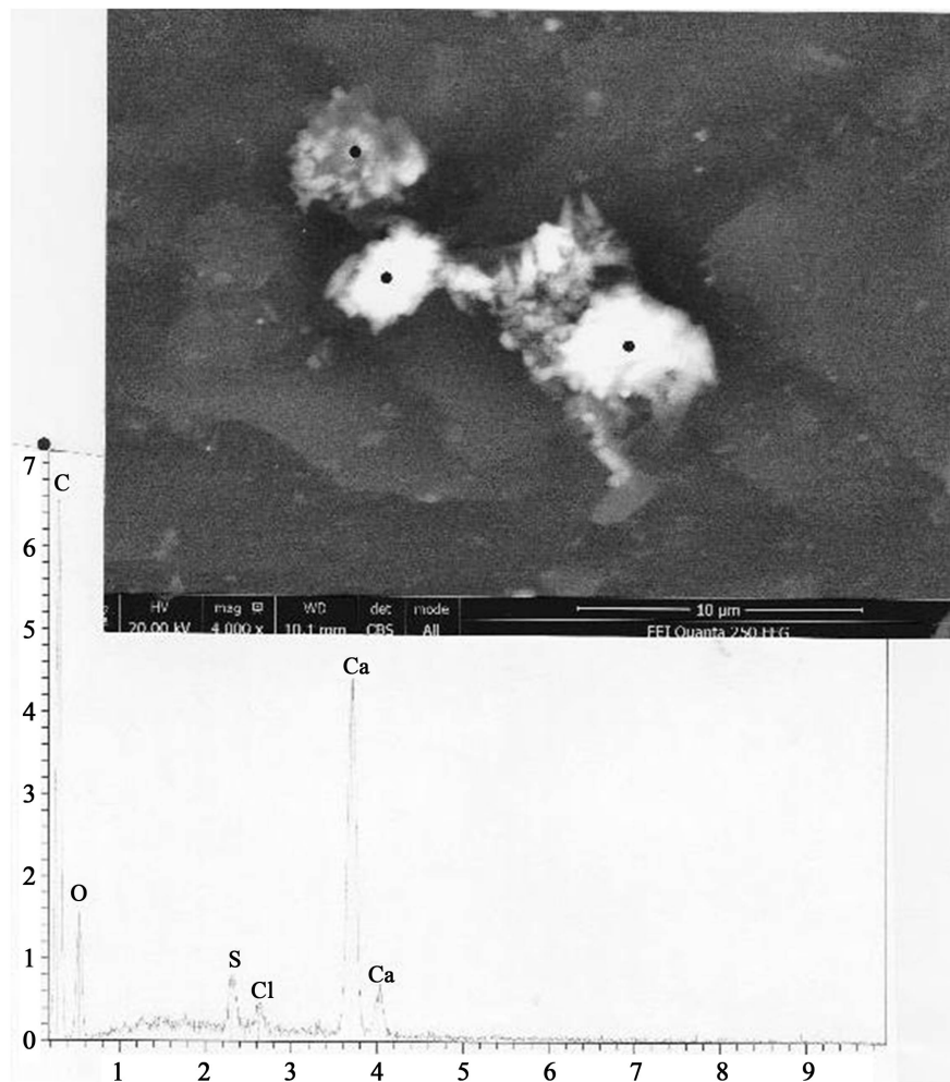
Figure 14. Above: SEM photograph (in CBS, 4000×) of a group of six coccoliths located on another portion of hair number 2. Below: common spectrum (at little black dots) of three of them.
