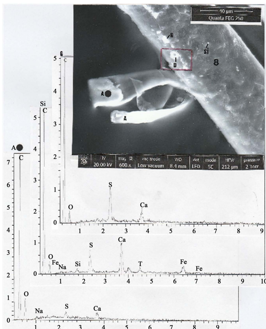
Figure 1. Above: a SEM photograph (in LFD, 600×) of the marine island located on hair number 8. G: a gypsum particle; Si: a silice particle; D: a diatom (the red rectangle area is enlarged in a following figure); A: two parts of the thalle of an algae. The black dot in the algae superior part indicates the location where elemental analyses are realized. Below: the spectras. Upper spectrum: that of the G particle; medium spectrum: that of the Si particle; lower spectrum: that of the A superior part. C: carbon; O: oxygen; Fe (three peaks): iron; Na: sodium; Si: silicium; S: sulphur; Ca (two peaks): calcium; Ti: titanium.
