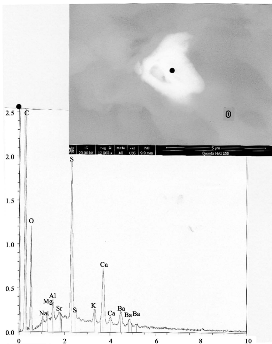
Figure 27. A second example of a barytine particle on hair number 1. Above: SEM photograph (in CBS, 12,000 \times ) of the barytine particle, located in another portion of hair number 1. Below: spectrum at the black dot.
