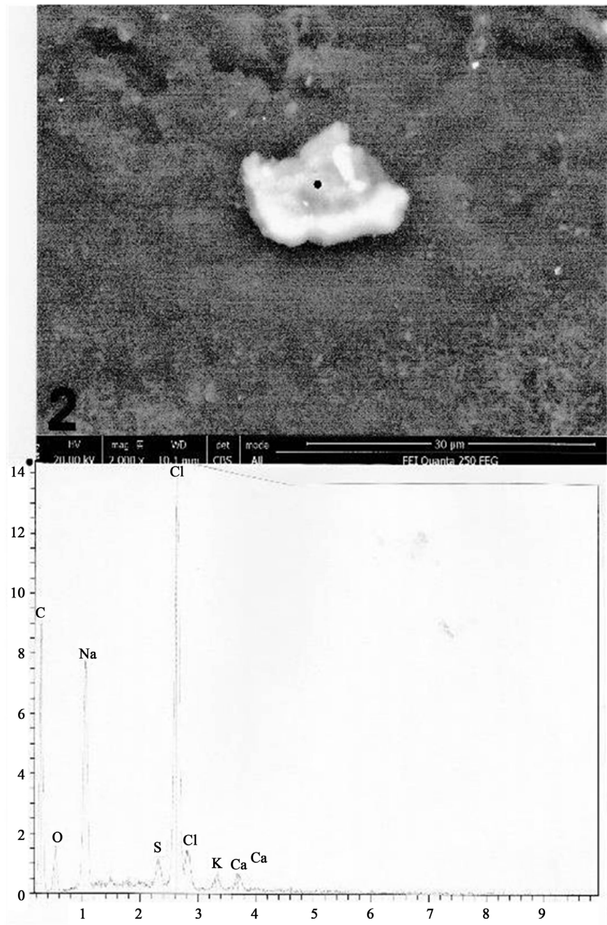
Figure 6. Another salt particle on the hair number 2. Above: SEM photograph (in CBS, 2000×) showing the particle. Below: spectrum at the little black dot. C: carbon; O: oxygen; Na: sodium; S: sulphur; Cl (two peaks): chlorine; K: potassium; Ca (two peaks): calcium.
