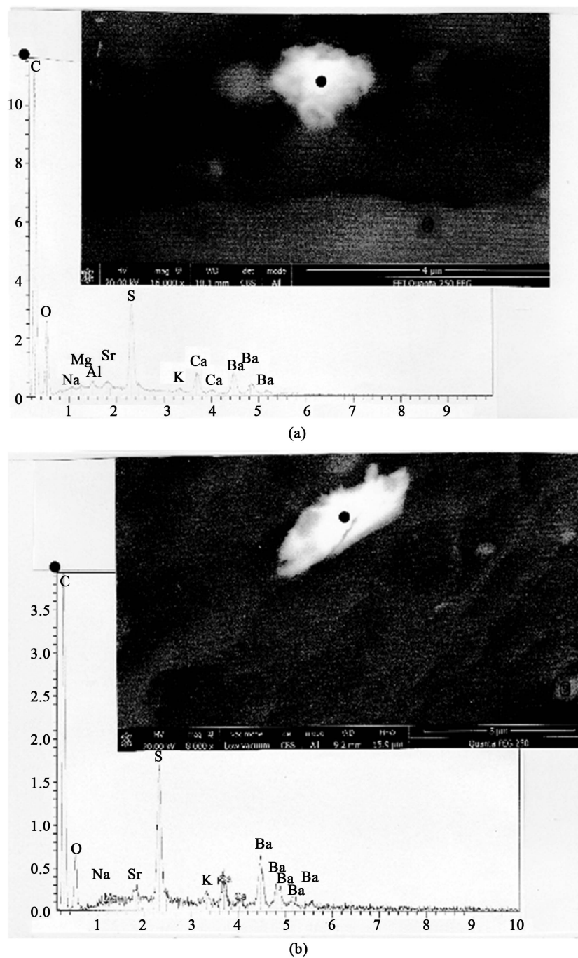
Figure 28. Third and fourth examples of barytine particles at the vicinity of hair number 2 and on the hair number 9. (a): upper SEM photograph (in CBS, 16,000 \times ) of the third barytine particle located at the vicinity of a portion of hair number 2. Below: spectrum at the black dot; (b): lower SEM photograph (in CBS, 8000 \times ) of the fourth barytine particle located on a portion of hair number 9. Below: spectrum at the black dot.
