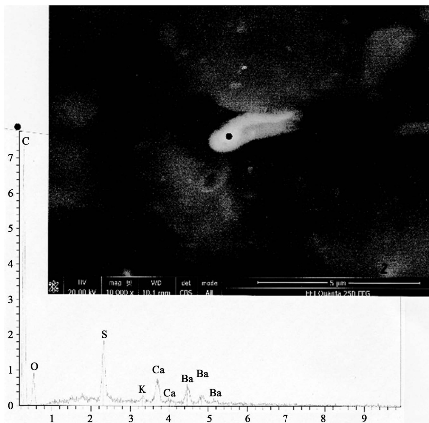
Figure 29. A micro-trail of barium sulphate pigment on hair number 2. Above: SEM photograph (in CBS, 10,000×) of the micro-trail, located at some part of the hair number 2 surface. Below: spectrum at the black dot. C: carbon; O: oxygen; S: sulphur; K: potassium; Ca (two peaks): calcium; Ba (three peaks): barium.
