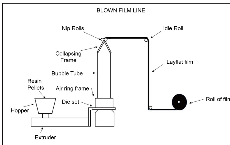
Figure 2. Blown film extrusion line flowsheet.
